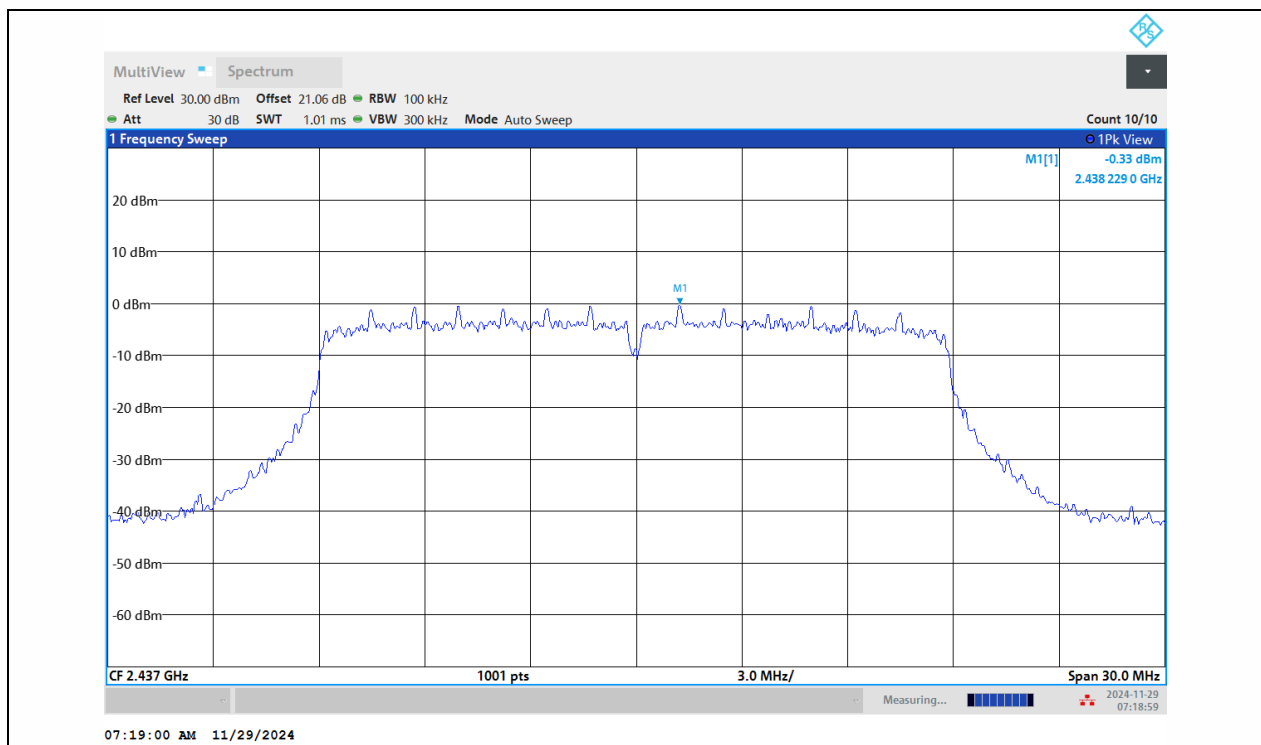
11N20MIMO-Ant1-2437-0-Reference-PASS
