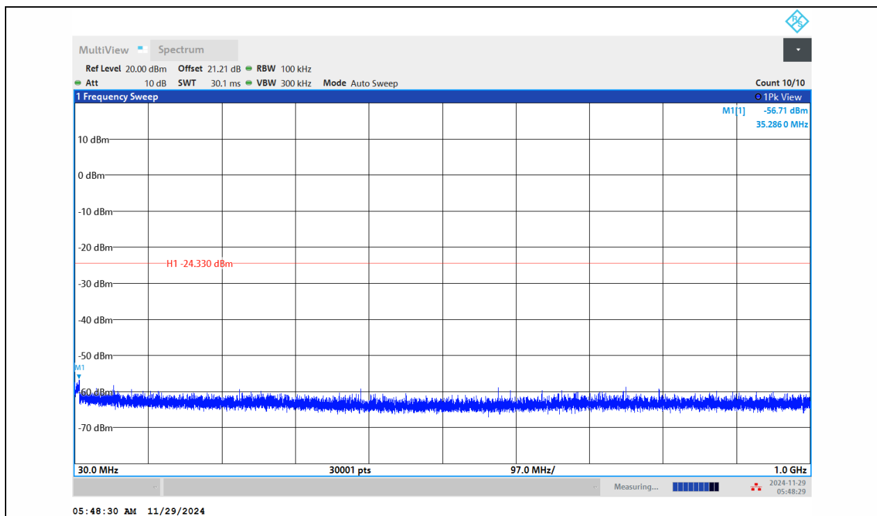
11B-Ant1-2412-30~1000-PASS
