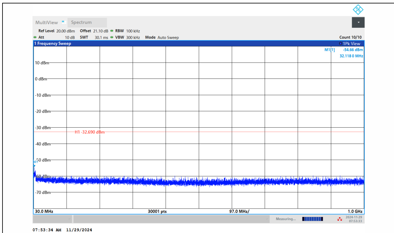
11N40MIMO-Ant1-2422-30~1000-PASS
