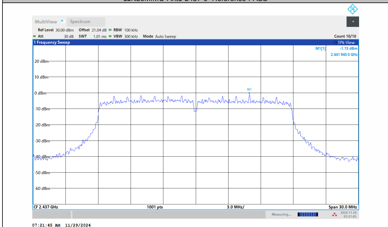
11N20MIMO-Ant2-2437-0-Reference-PASS
