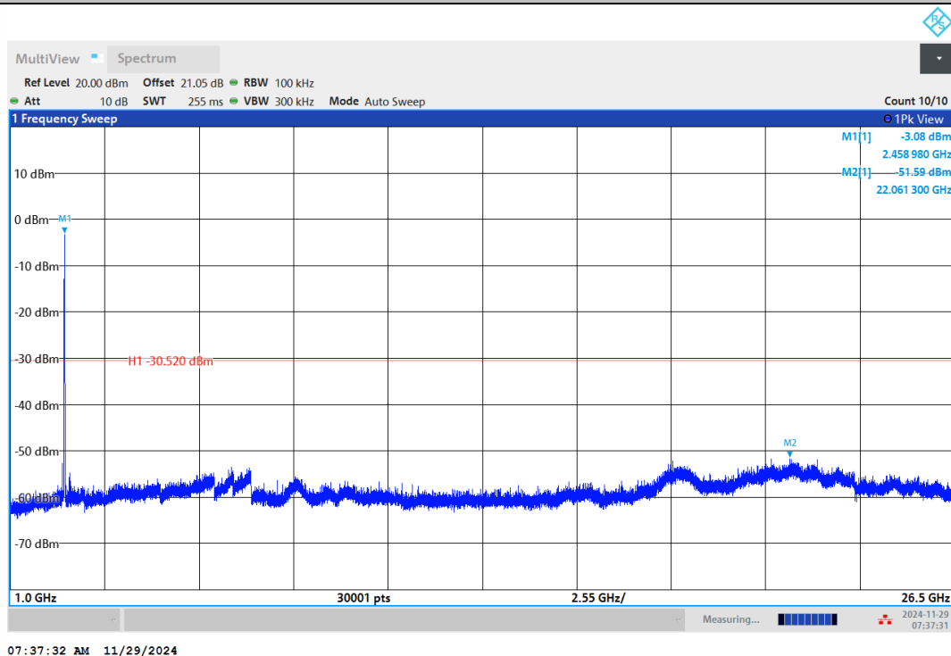
11N20MIMO-Ant2-2462-1000~26500-PASS
