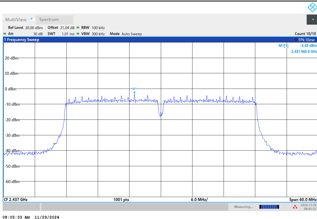
11N40MIMO-Ant2-2437-0-Reference-PASS
