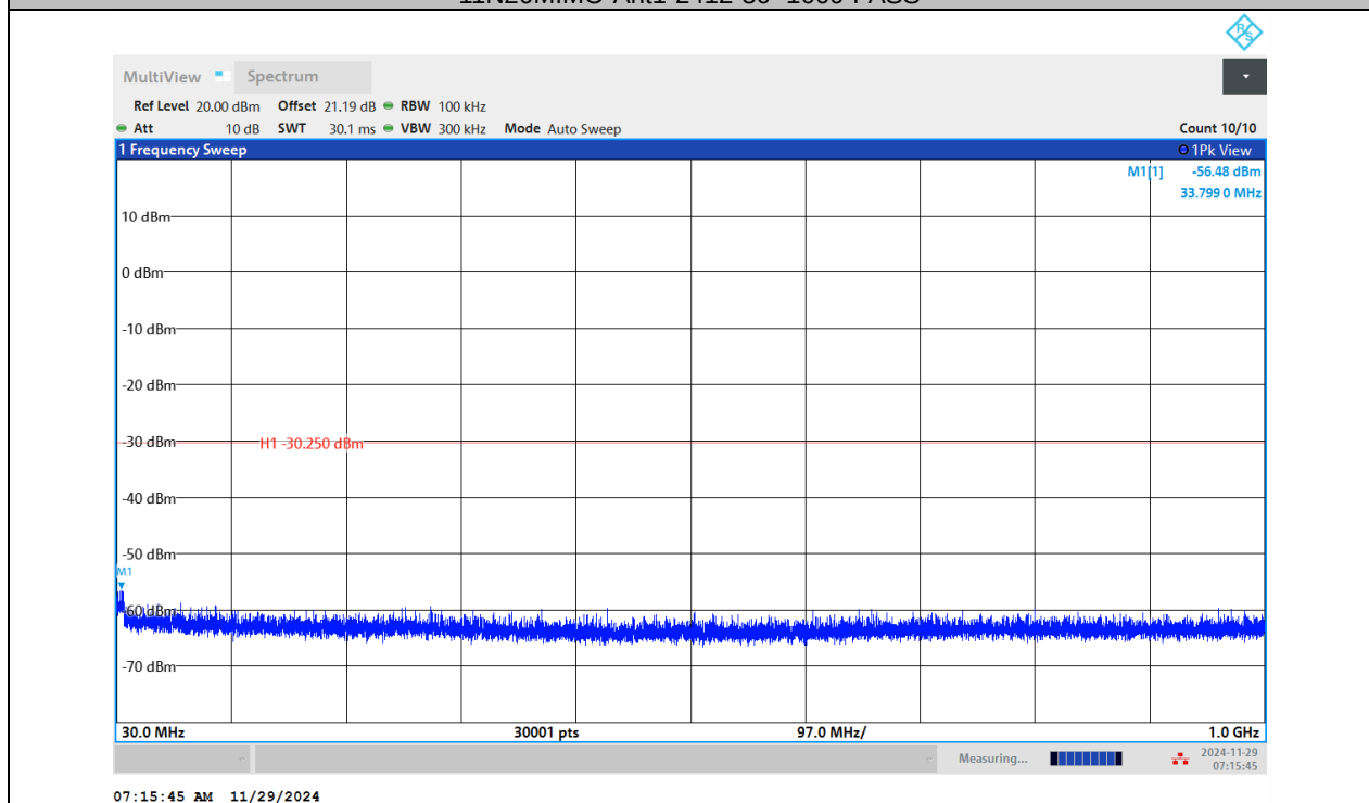
11N20MIMO-Ant2-2412-30~1000-PASS
