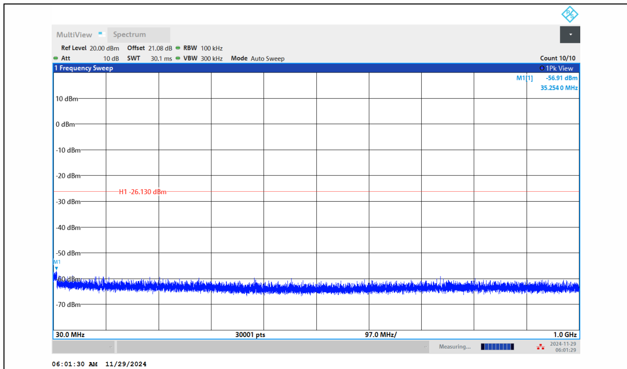
11B-Ant1-2462-30~1000-PASS
