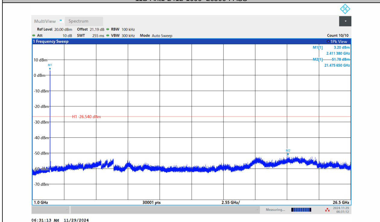
11B-Ant2-2412-1000~26500-PASS
