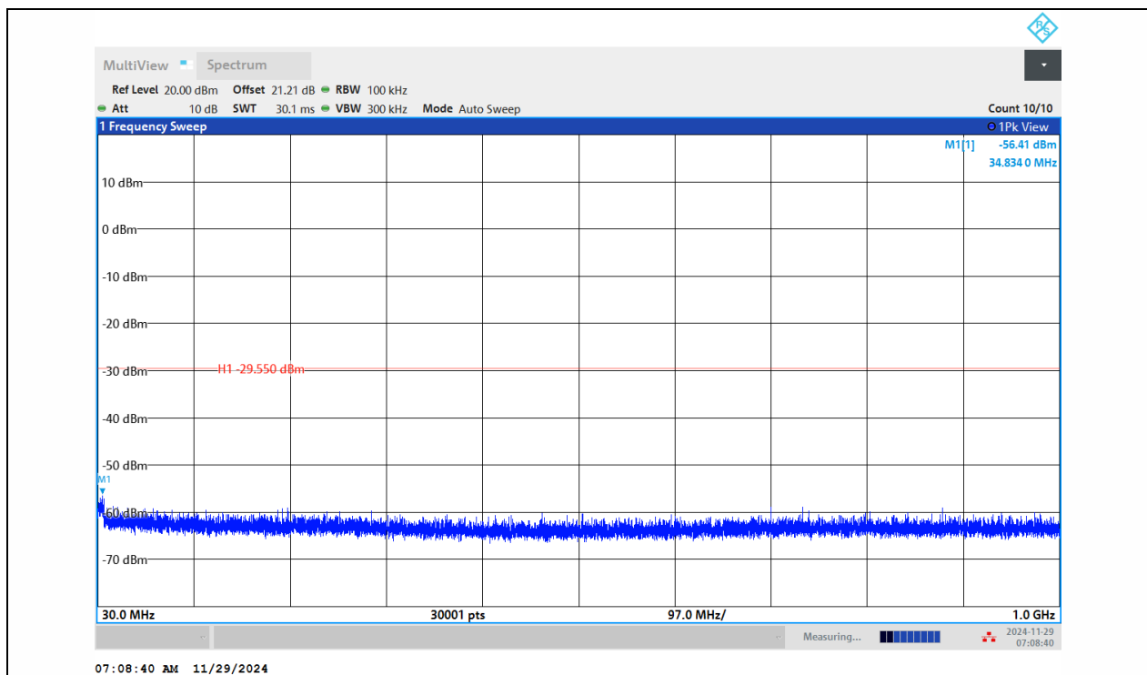
11N20MIMO-Ant1-2412-30~1000-PASS
