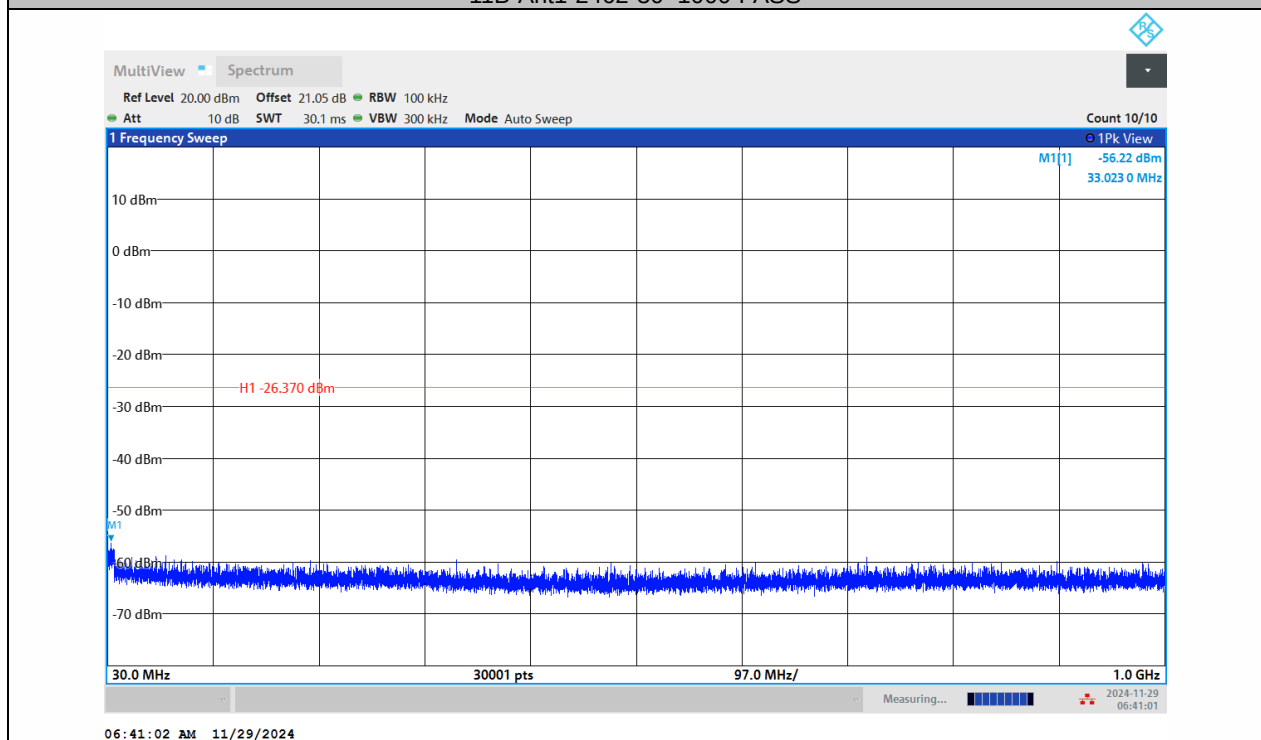
11B-Ant2-2462-30~1000-PASS
