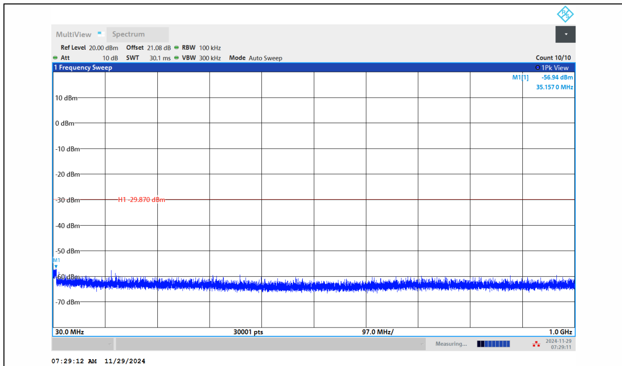
11N20MIMO-Ant1-2462-30~1000-PASS
