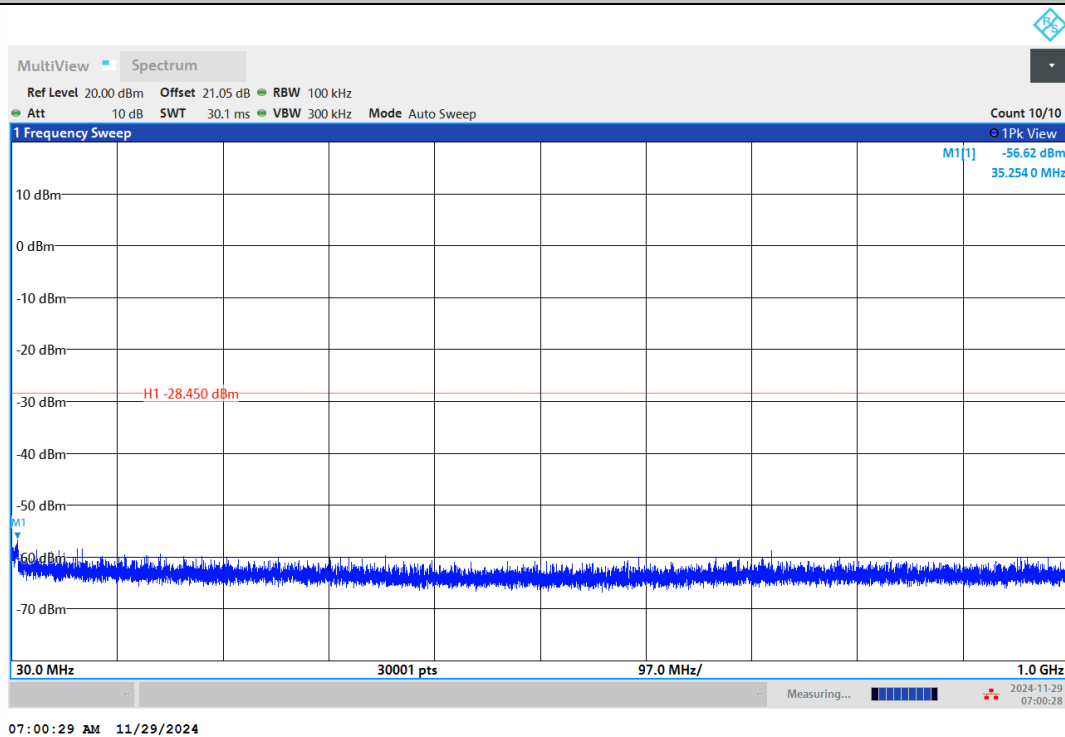
11G-Ant2-2462-30~1000-PASS
