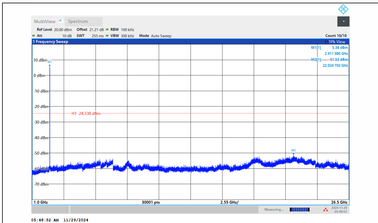
11B-Ant1-2412-1000~26500-PASS
