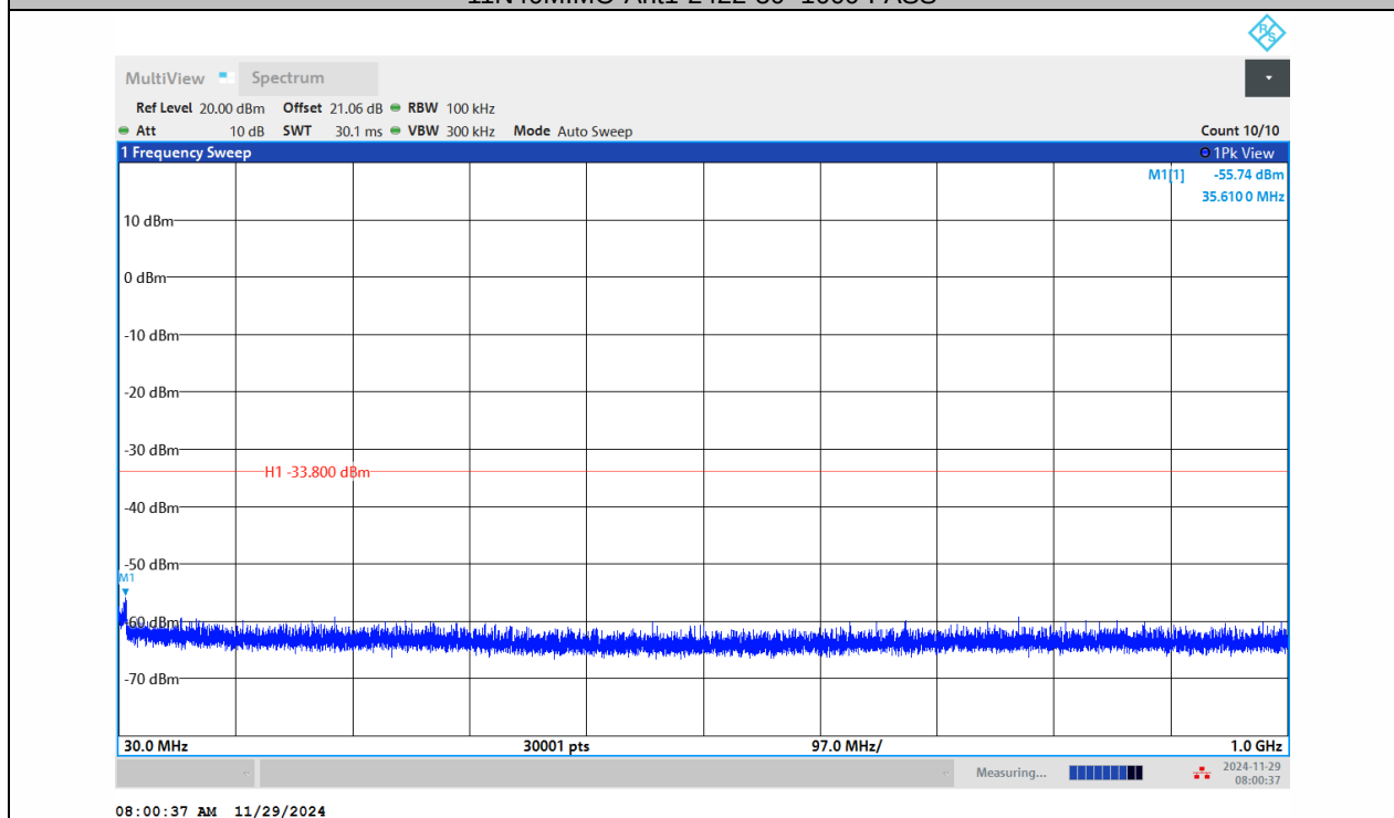
11N40MIMO-Ant2-2422-30~1000-PASS
