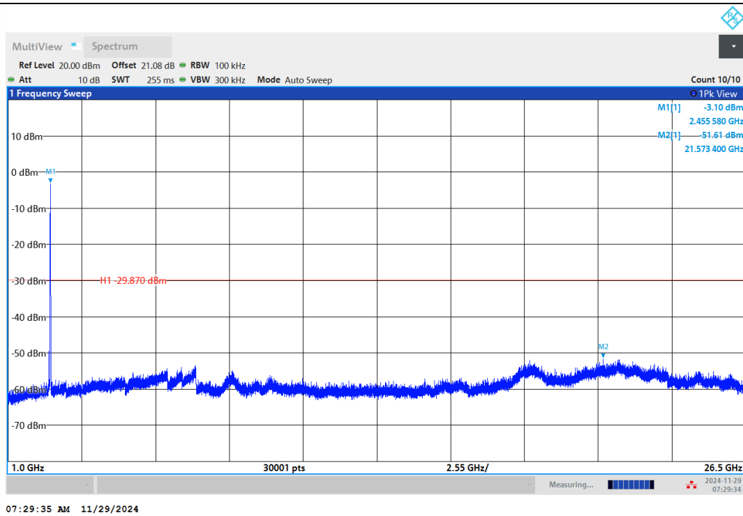
11N20MIMO-Ant1-2462-1000~26500-PASS
