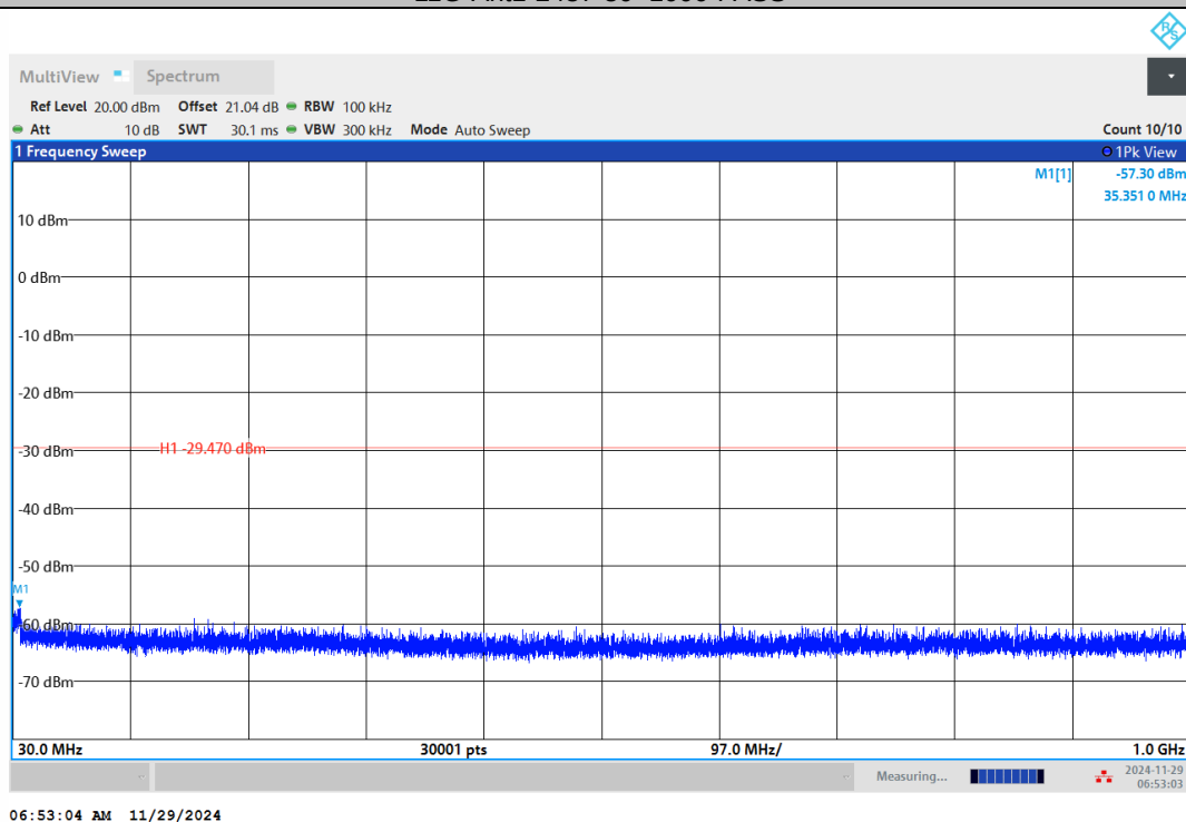
11G-Ant2-2437-30~1000-PASS
