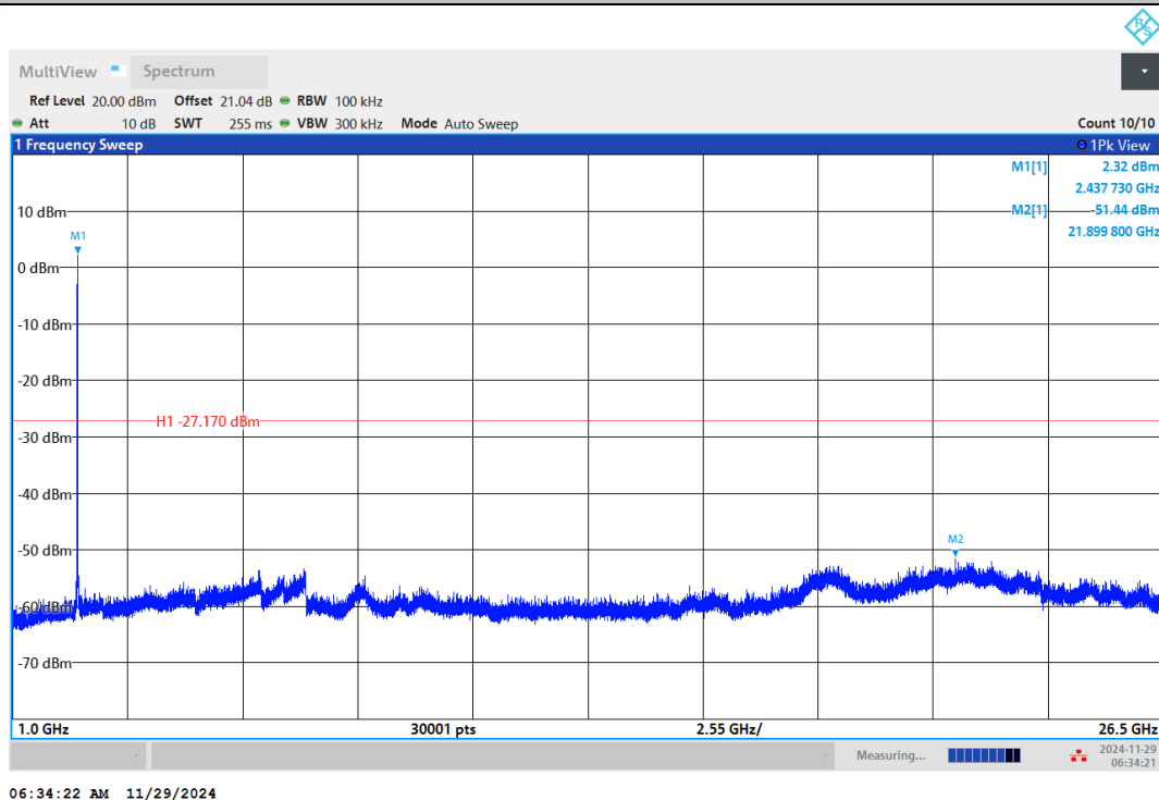
11B-Ant2-2437-1000~26500-PASS
