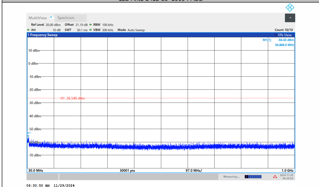
11B-Ant2-2412-30~1000-PASS
