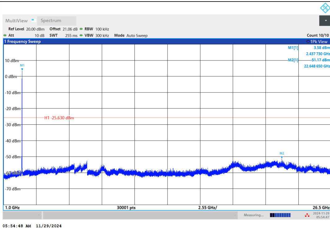
11B-Ant1-2437-1000~26500-PASS
