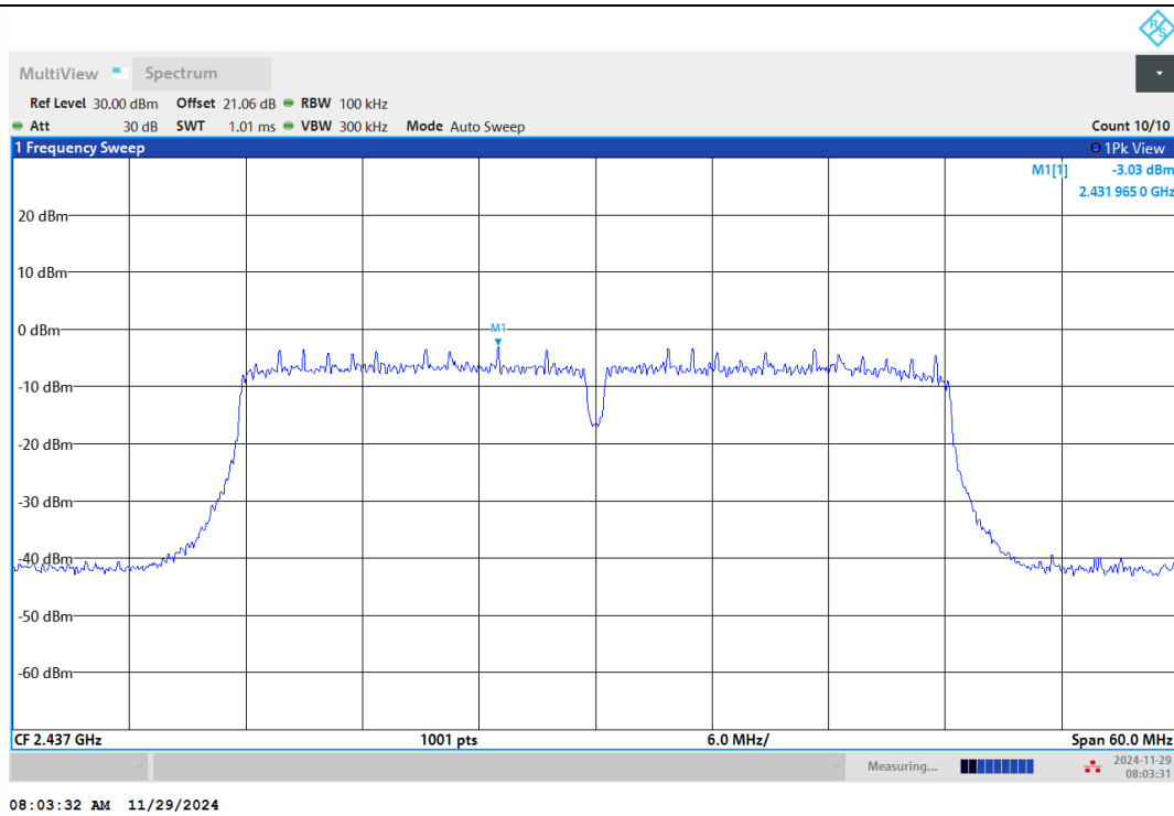
11N40MIMO-Ant1-2437-0-Reference-PASS
