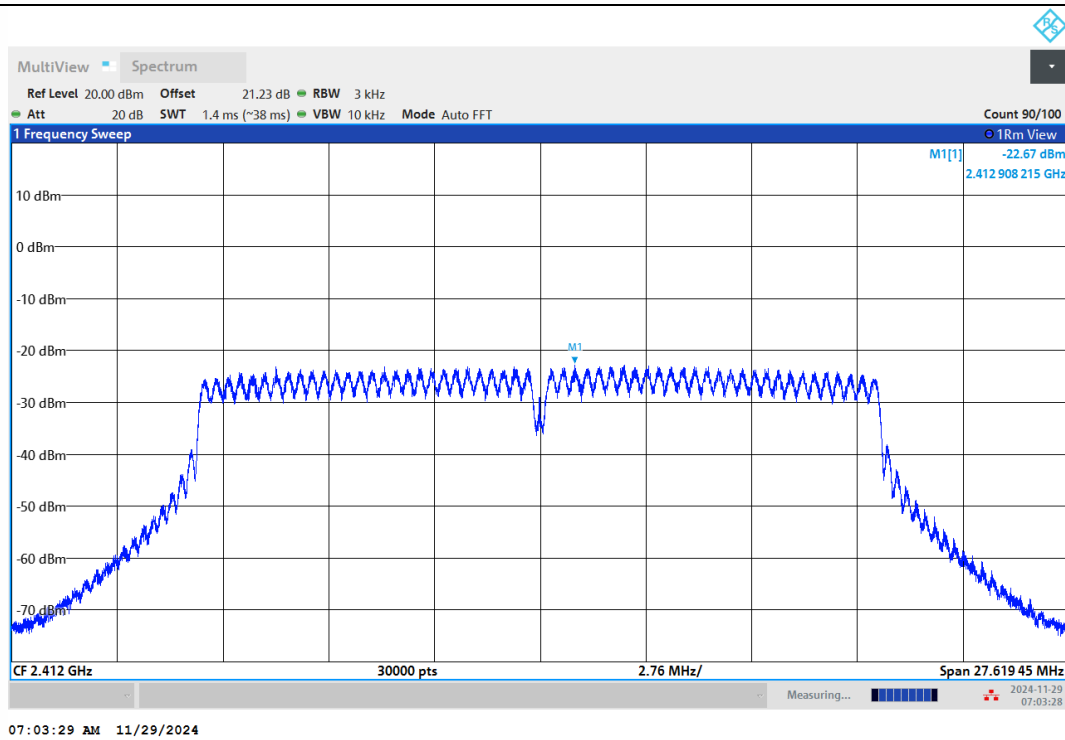
11N20MIMO-Ant1-2412-PASS
