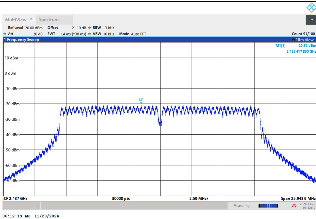
11G-Ant1-2437-PASS
