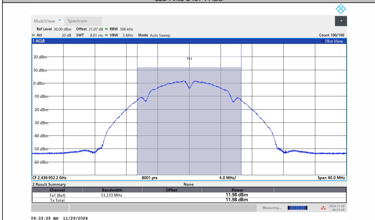
11B-Ant2-2437-PASS
