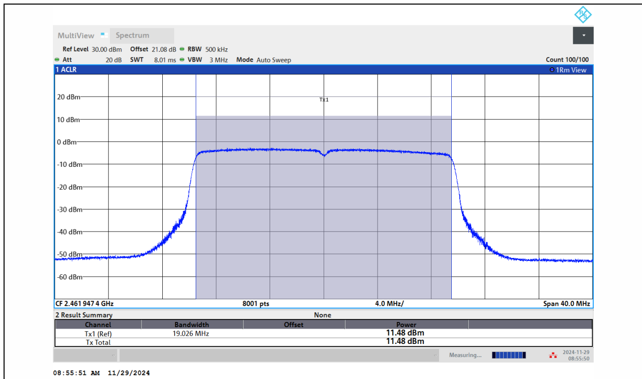
11AX20MIMO-Ant1-2462-PASS
