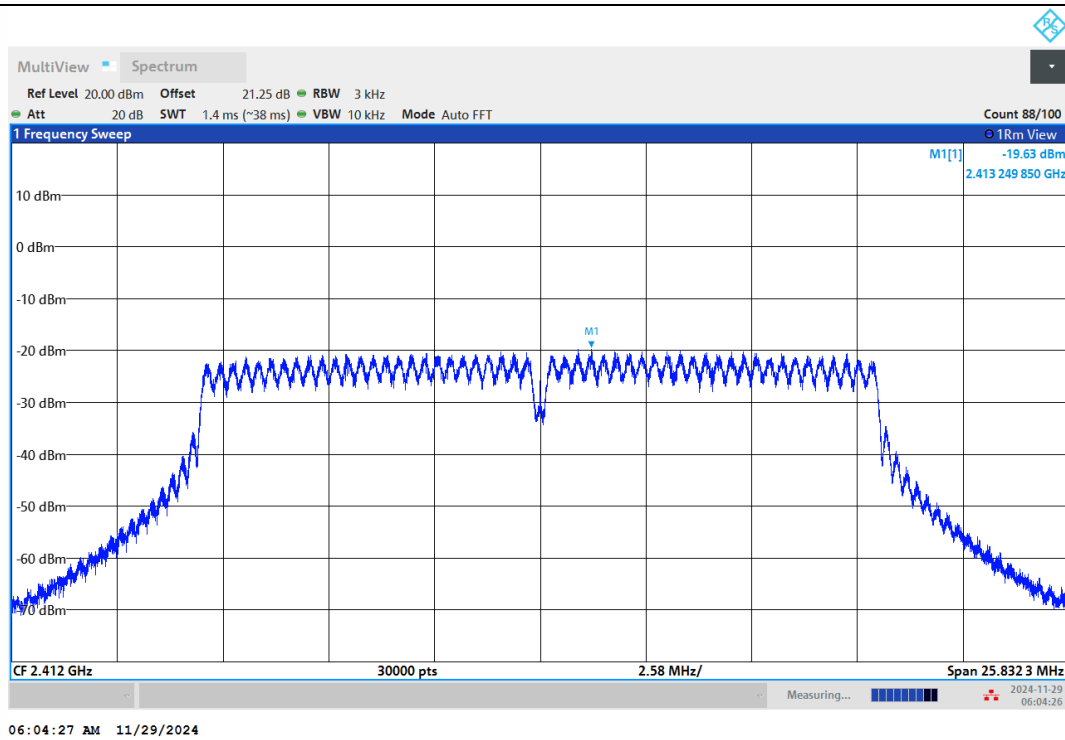
11G-Ant1-2412-PASS
