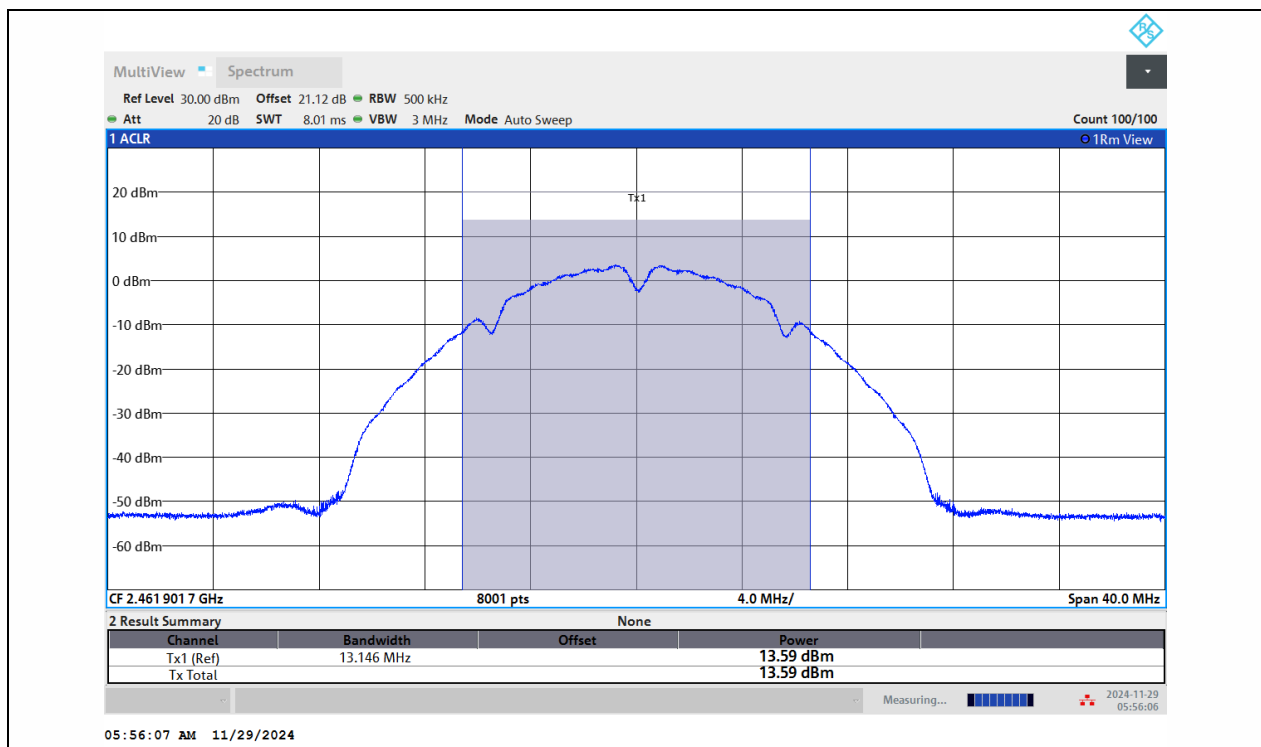
11B-Ant1-2462-PASS
