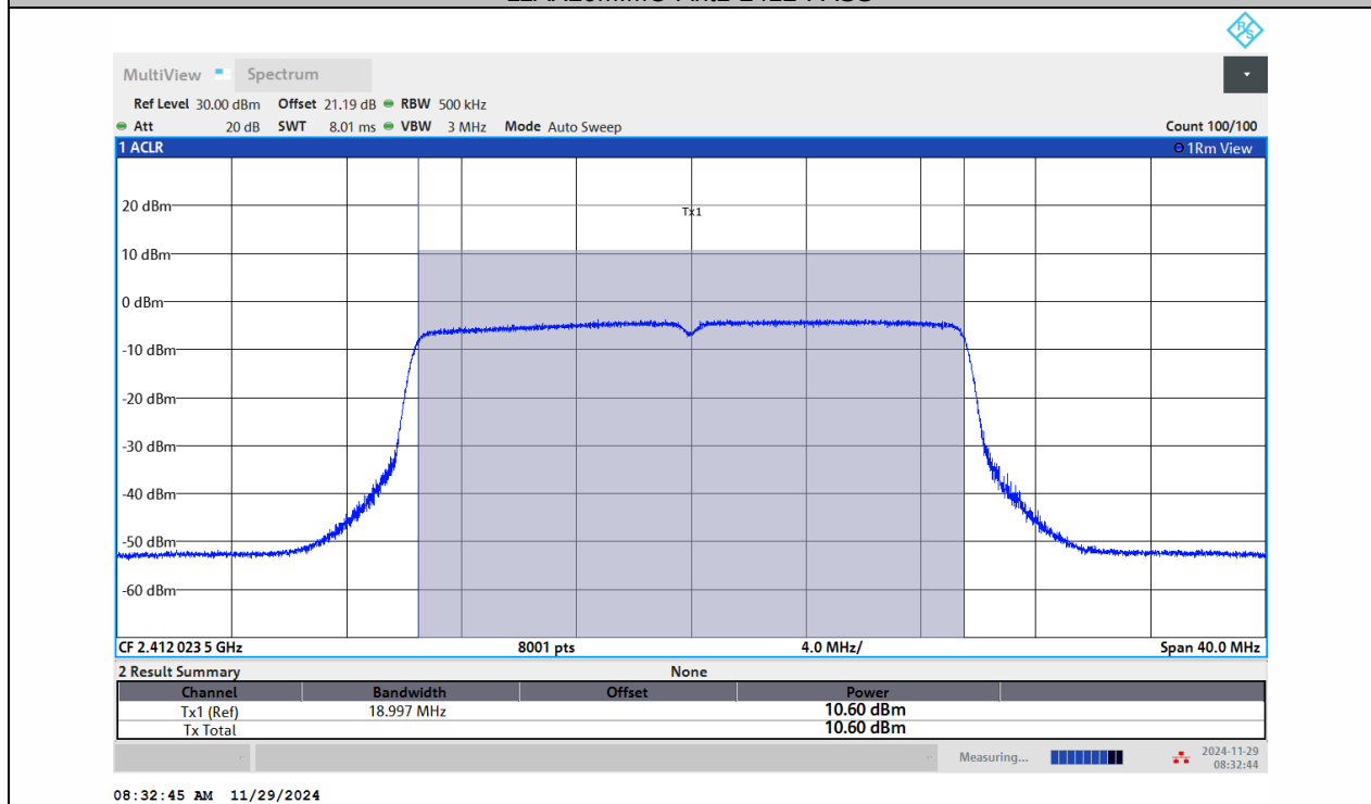
11AX20MIMO-Ant2-2412-PASS
