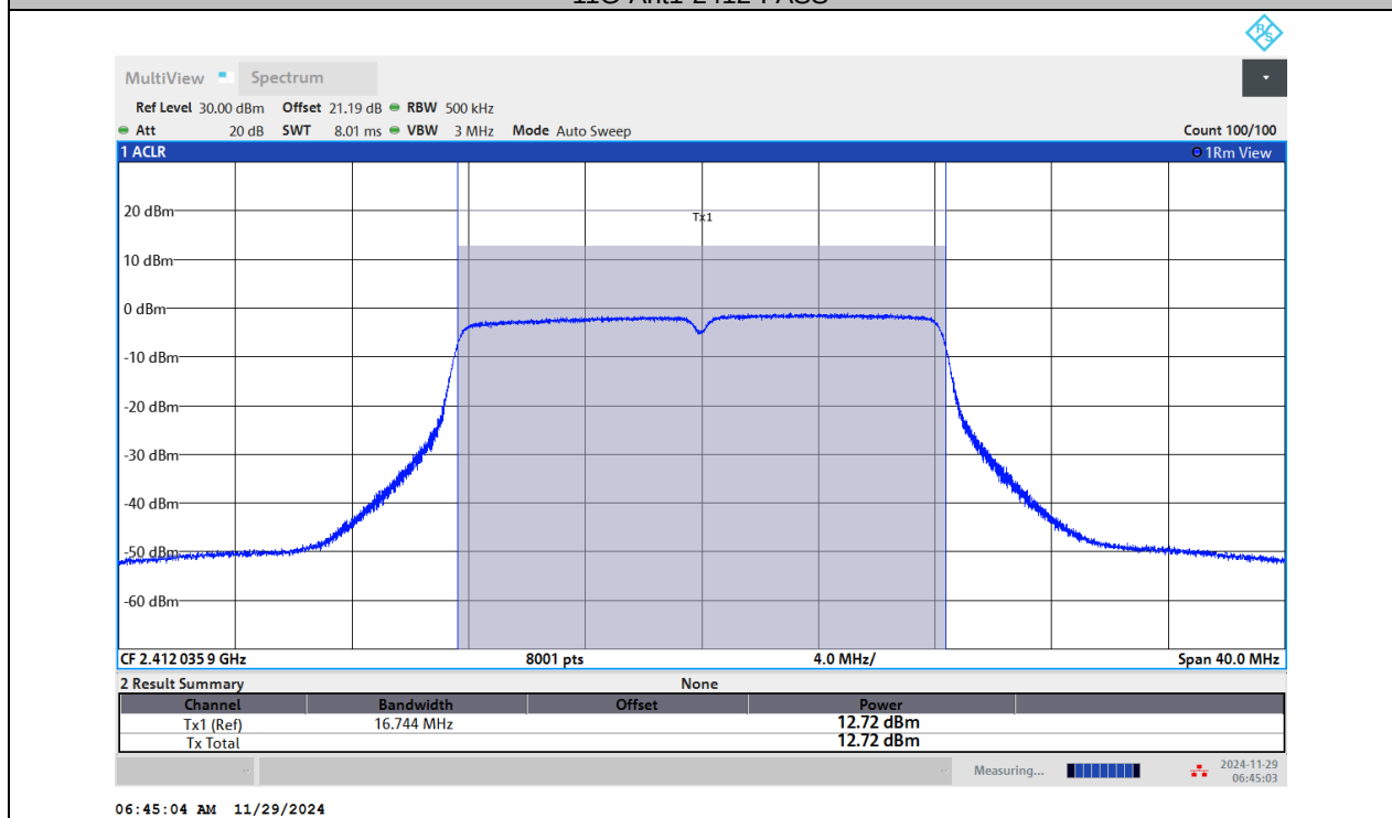
11G-Ant2-2412-PASS
