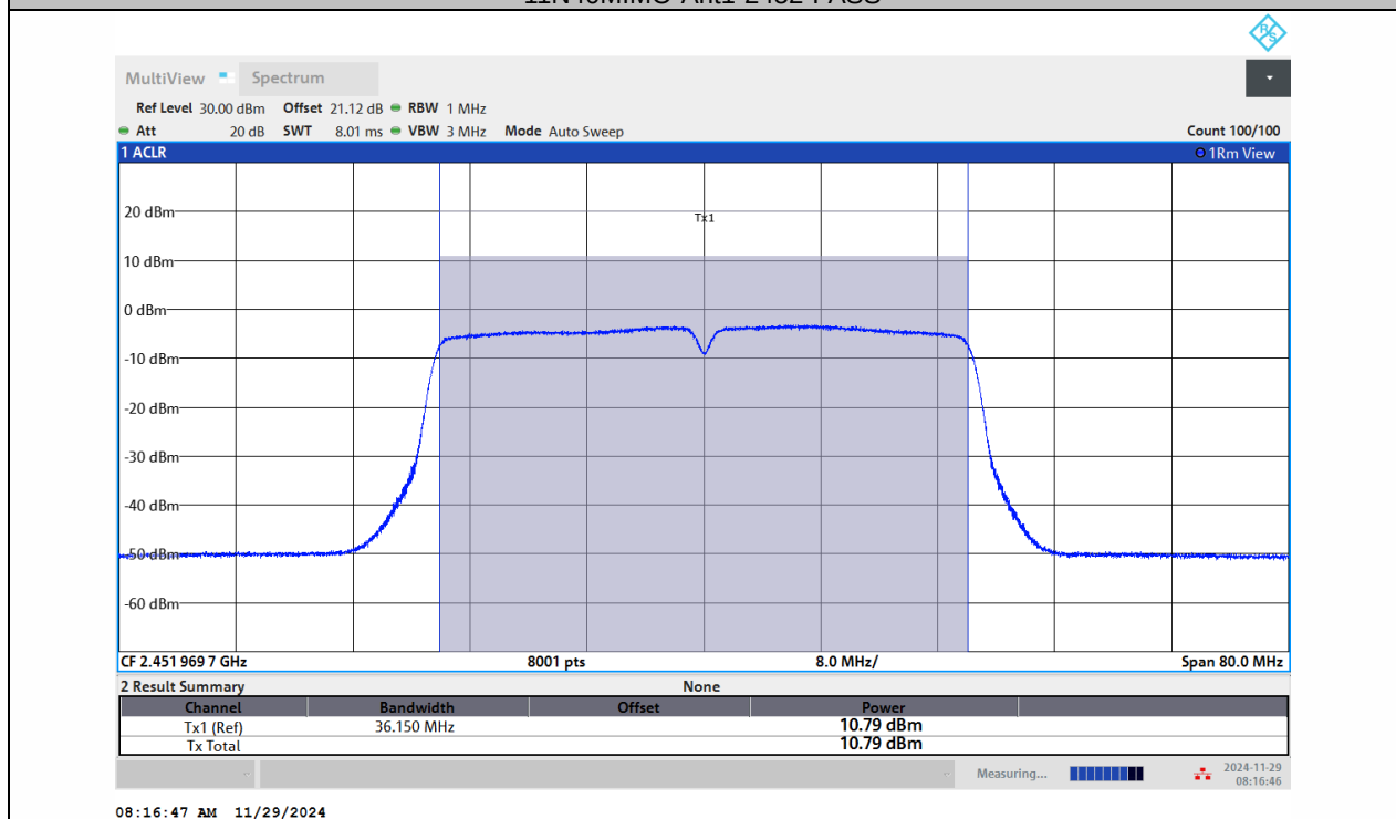
11N40MIMO-Ant2-2452-PASS
