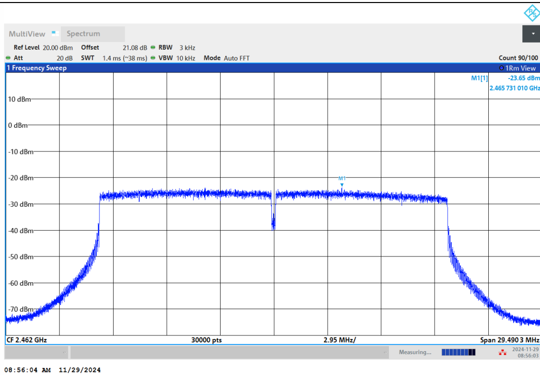
11AX20MIMO-Ant1-2462-PASS
