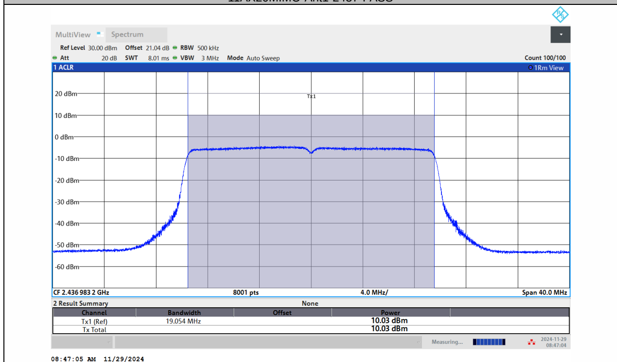
11AX20MIMO-Ant2-2437-PASS
