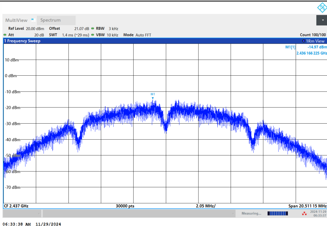
11B-Ant2-2437-PASS
