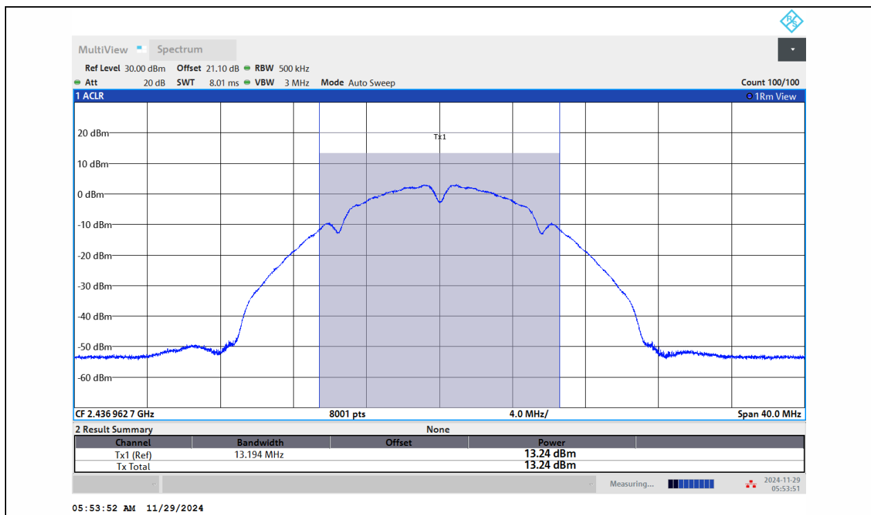
11B-Ant1-2437-PASS
