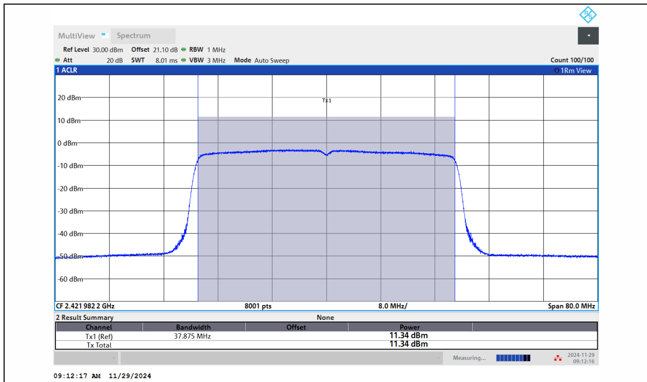
11AX40MIMO-Ant1-2422-PASS
