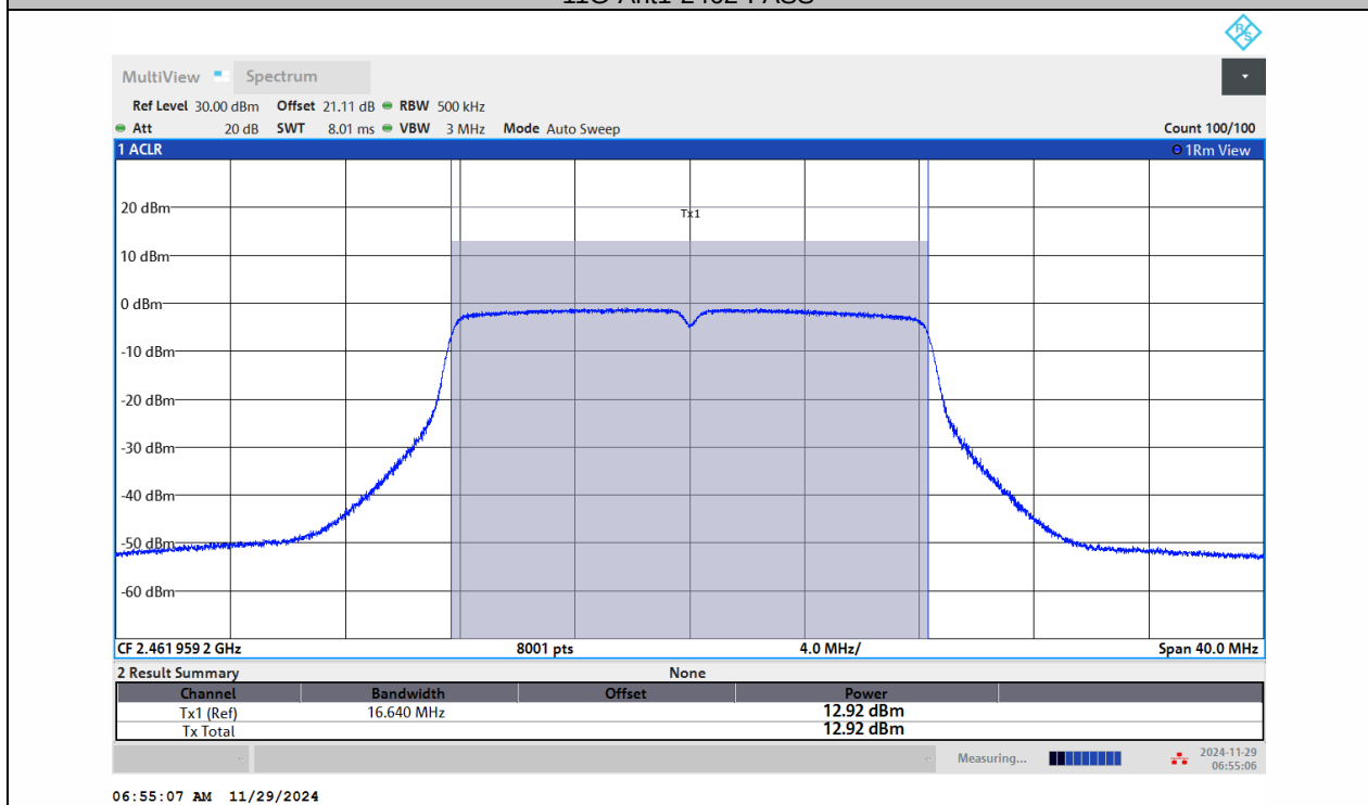
11G-Ant2-2462-PASS
