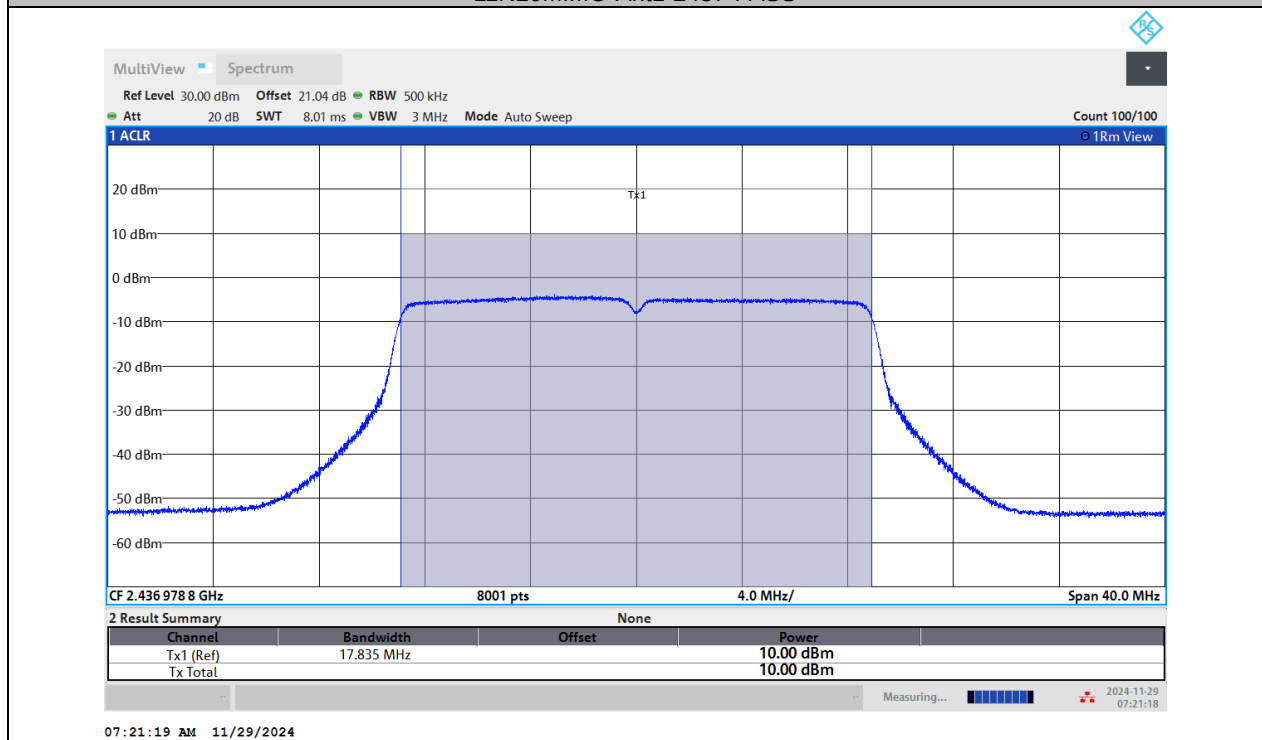
11N20MIMO-Ant2-2437-PASS
