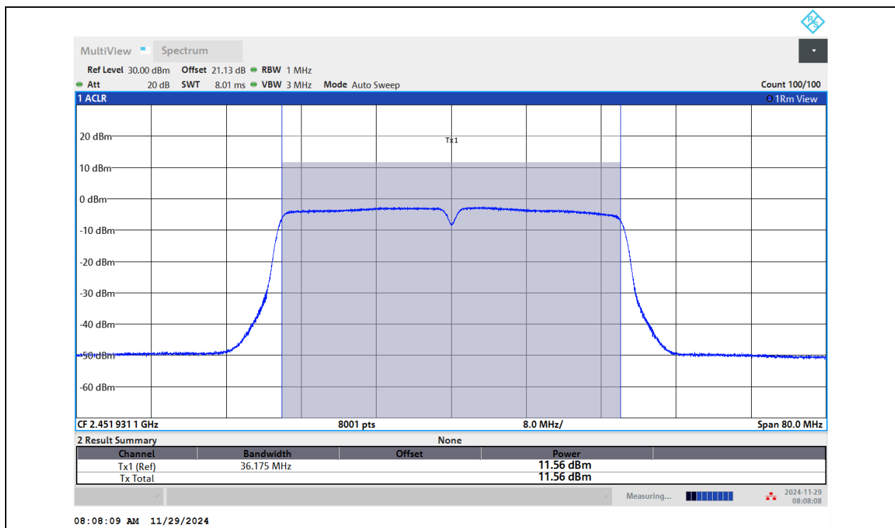
11N40MIMO-Ant1-2452-PASS
