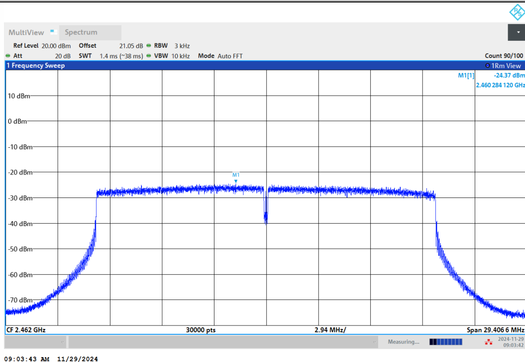
11AX20MIMO-Ant2-2462-PASS
