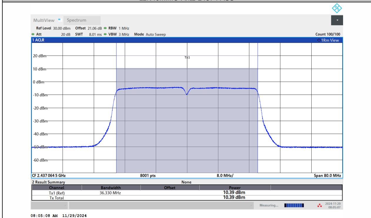
11N40MIMO-Ant2-2437-PASS
