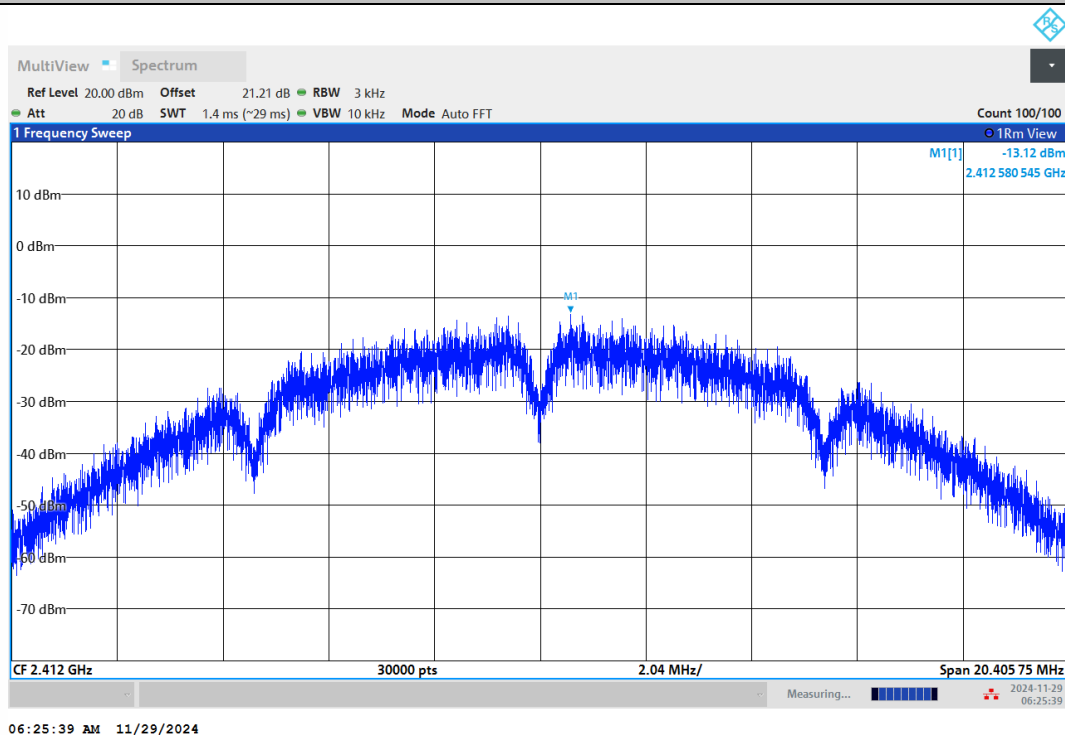
11B-Ant2-2412-PASS
