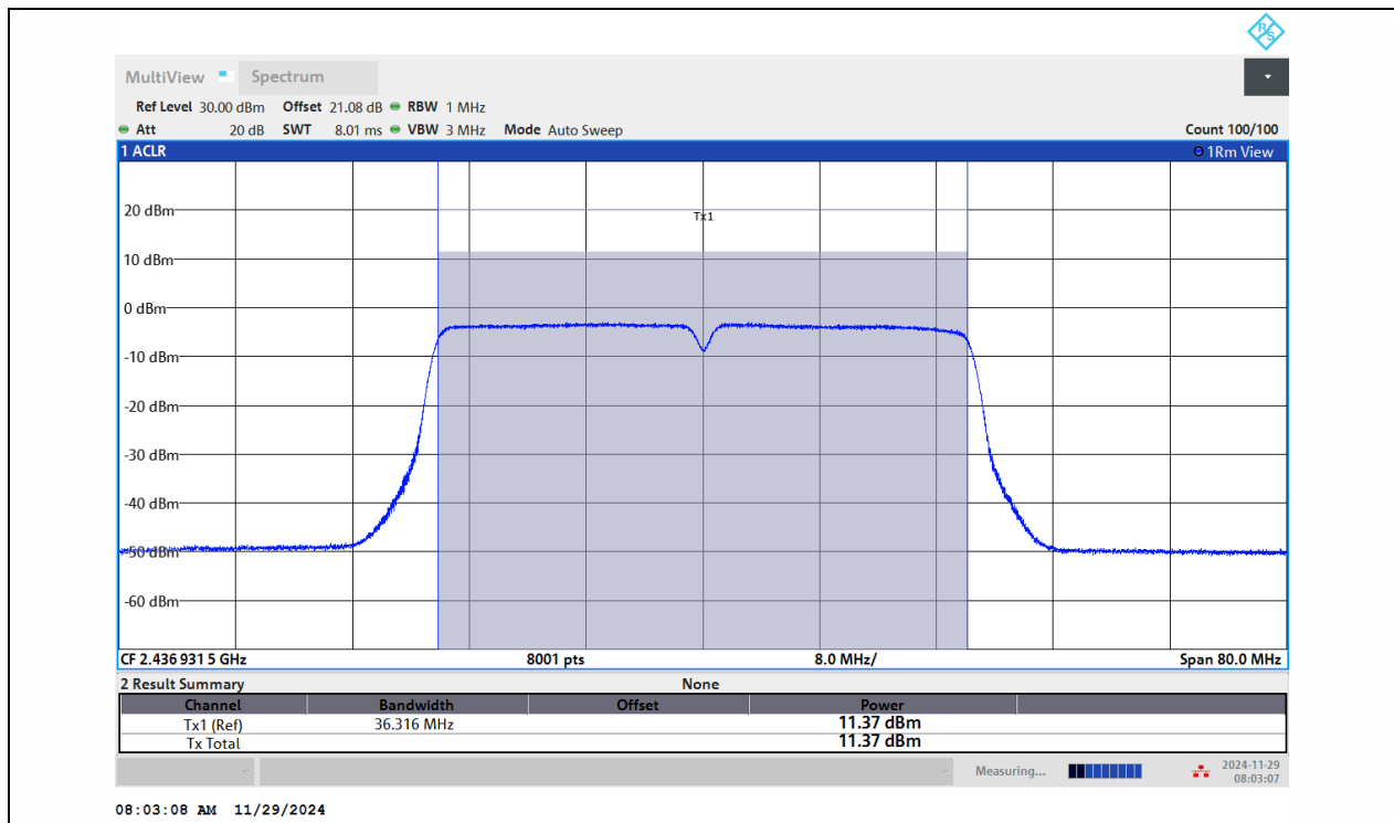
11N40MIMO-Ant1-2437-PASS
