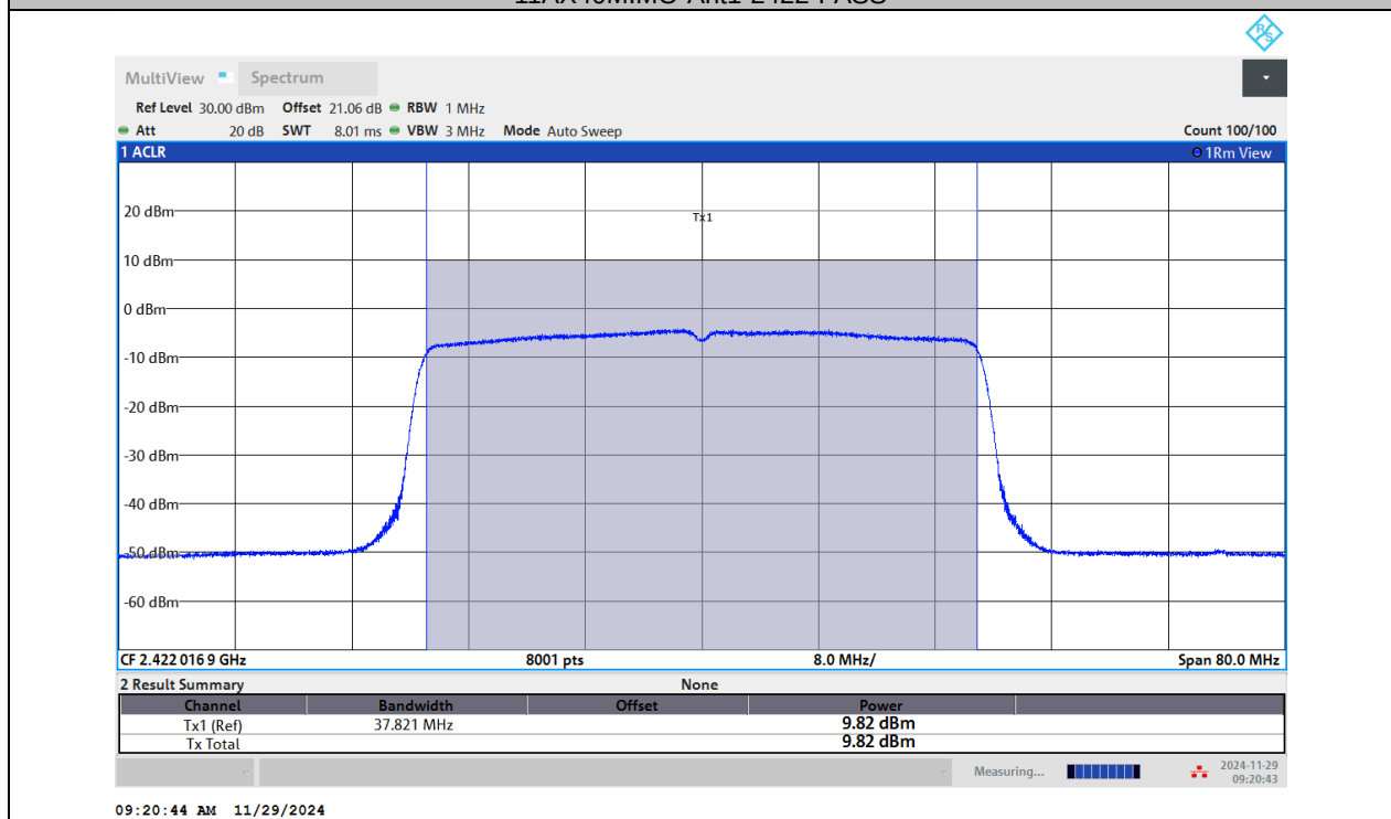
11AX40MIMO-Ant2-2422-PASS
