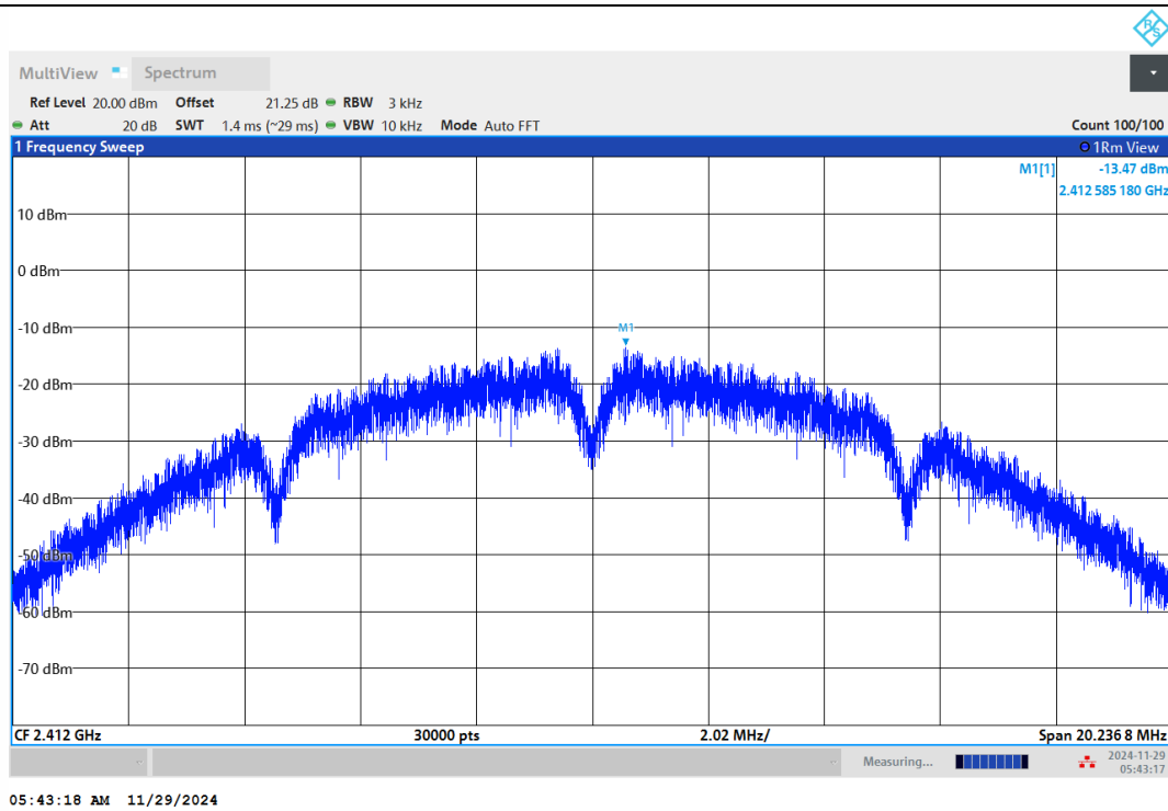
11B-Ant1-2412-PASS
