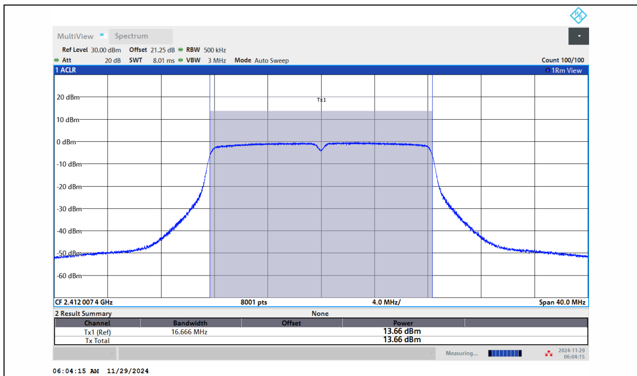
11G-Ant1-2412-PASS
