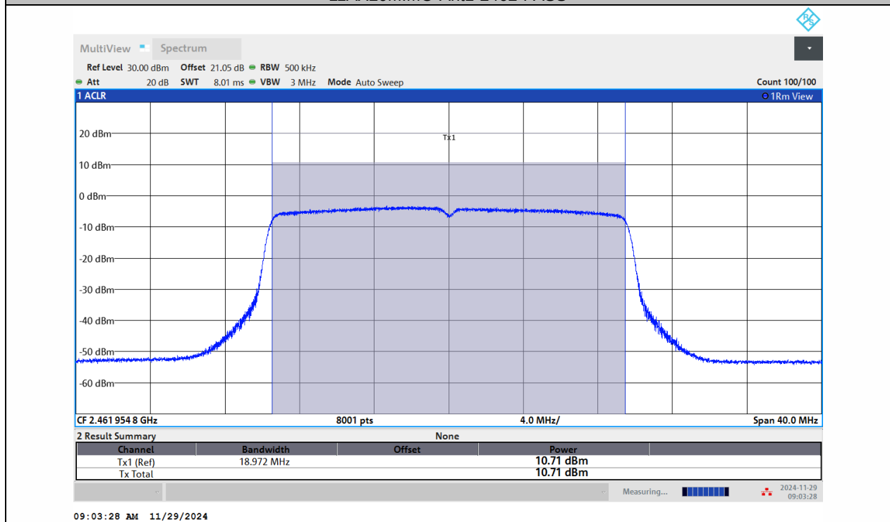
11AX20MIMO-Ant2-2462-PASS
