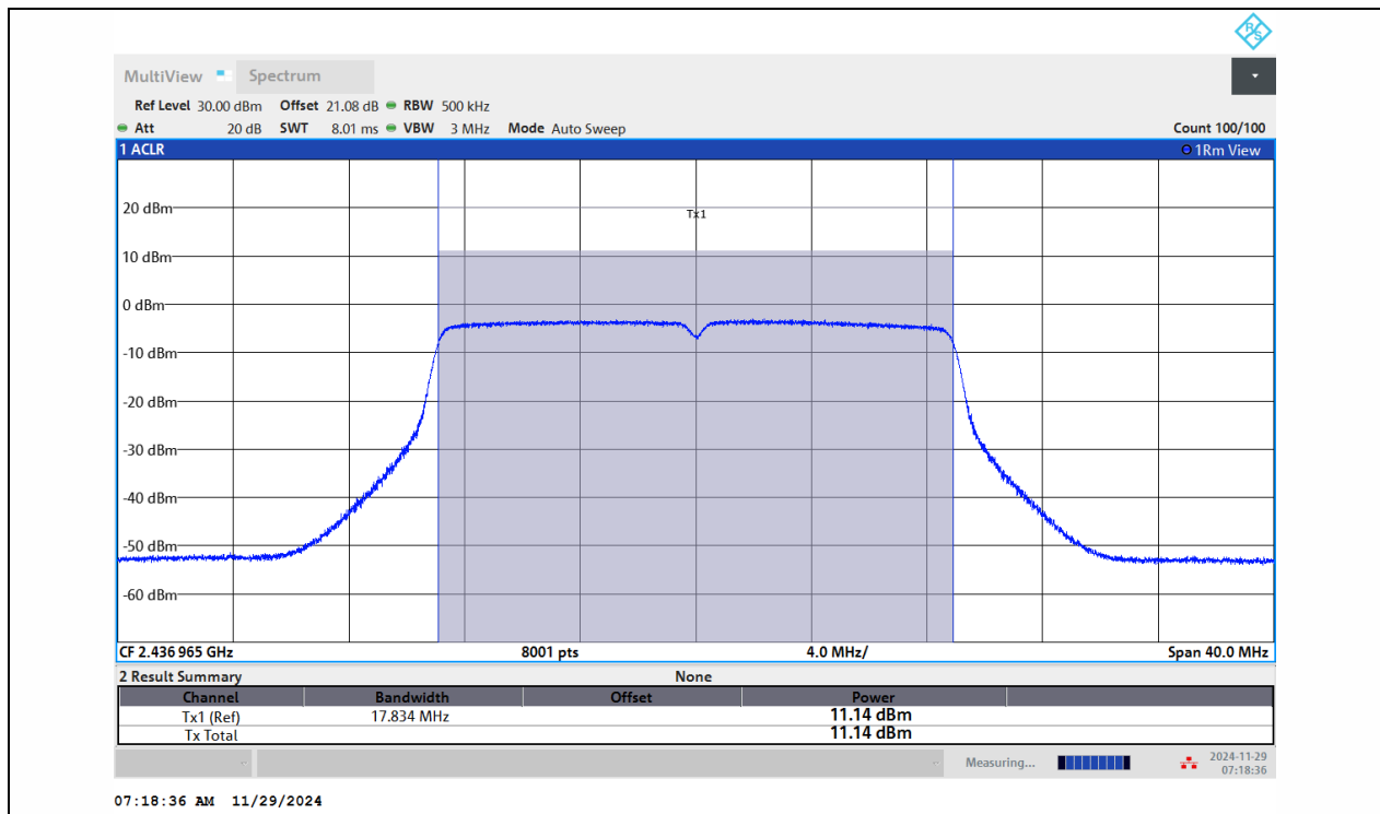
11N20MIMO-Ant1-2437-PASS
