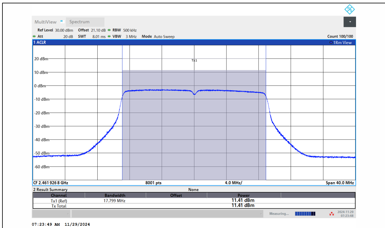
11N20MIMO-Ant1-2462-PASS
