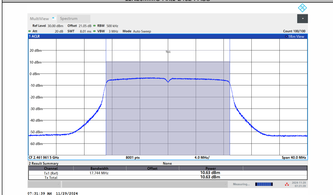
11N20MIMO-Ant2-2462-PASS
