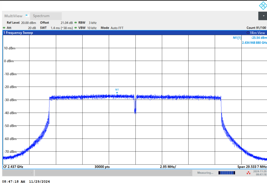
11AX20MIMO-Ant2-2437-PASS
