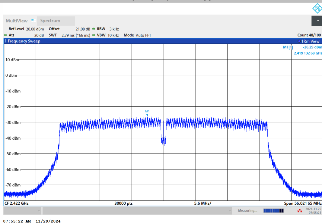
11N40MIMO-Ant2-2422-PASS
