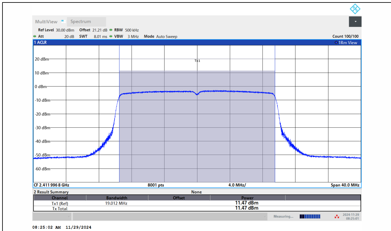
11AX20MIMO-Ant1-2412-PASS
