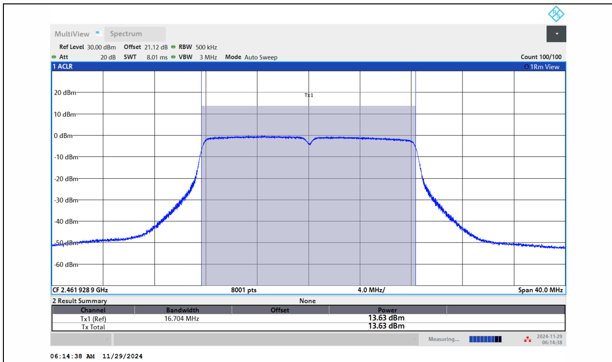
11G-Ant1-2462-PASS
