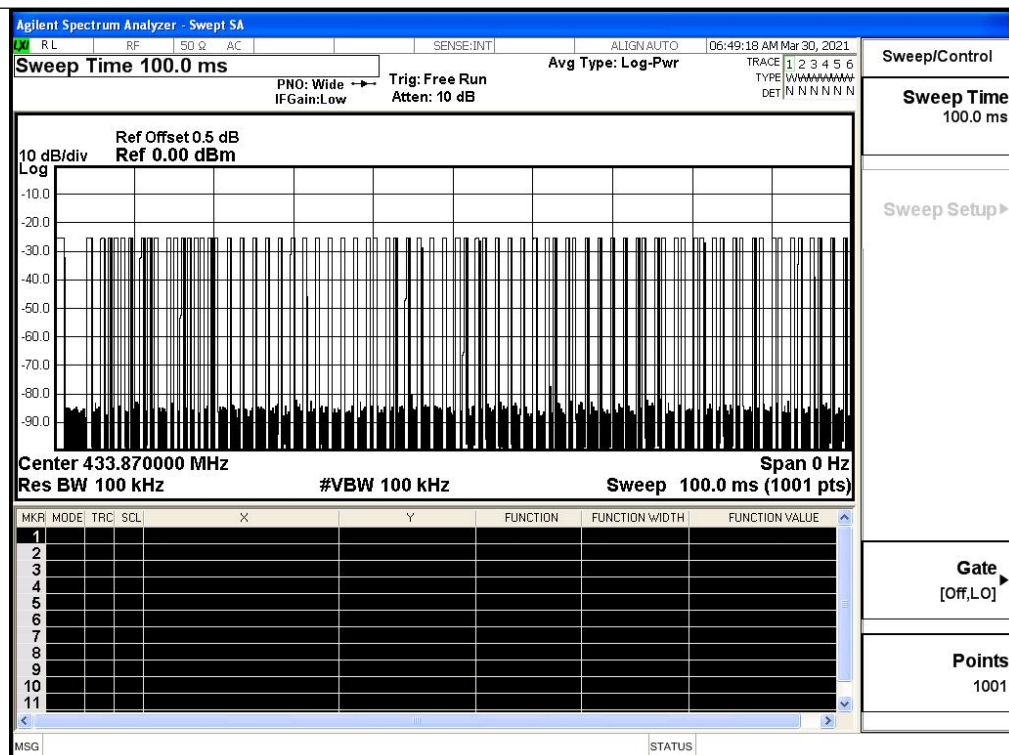
(Fig.3: capture the greatest amount of pulse "ON time" over 100 ms) Pluse type number=75
