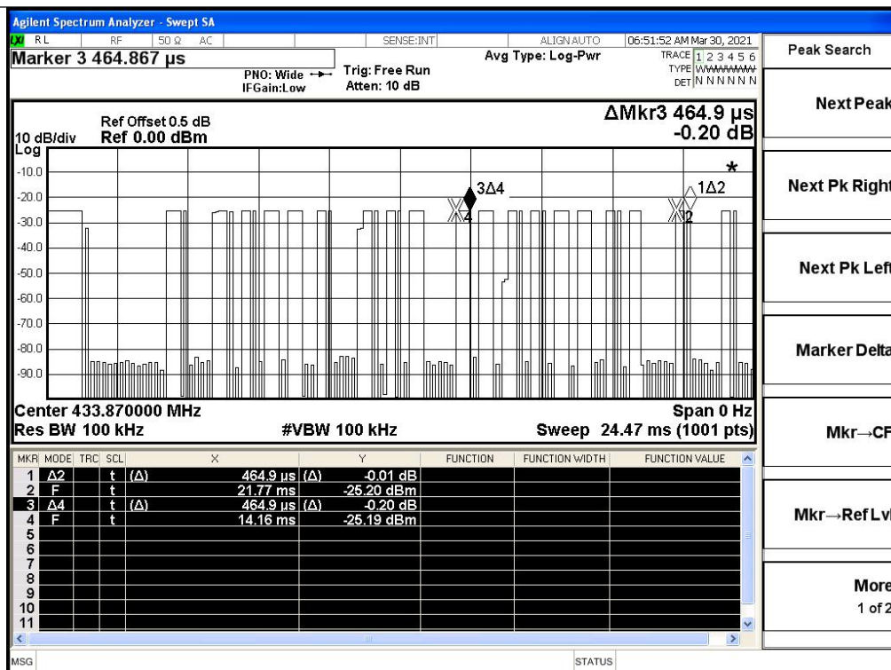
(Fig.4: Fig.4: pulse "ON time" for per pulse train) Pluse type width=0.4649ms
