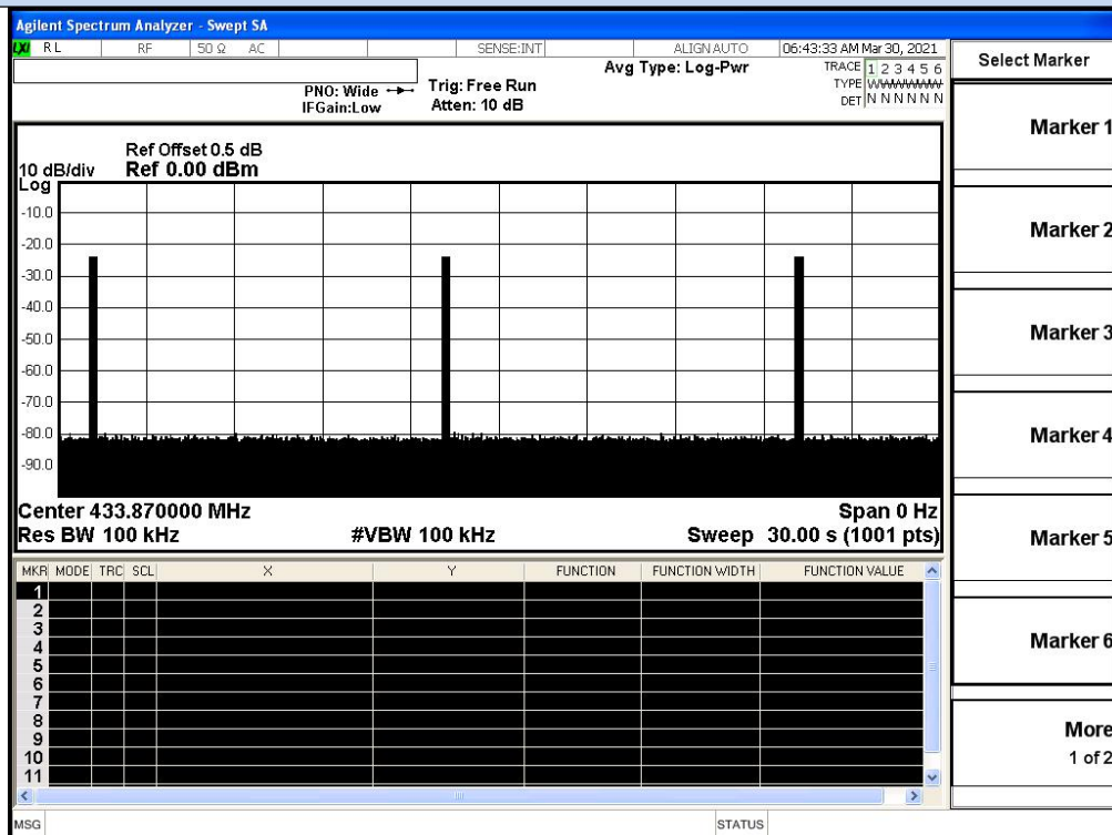
Fig.1(Periodic transmissions at regular predetermined intervals)
