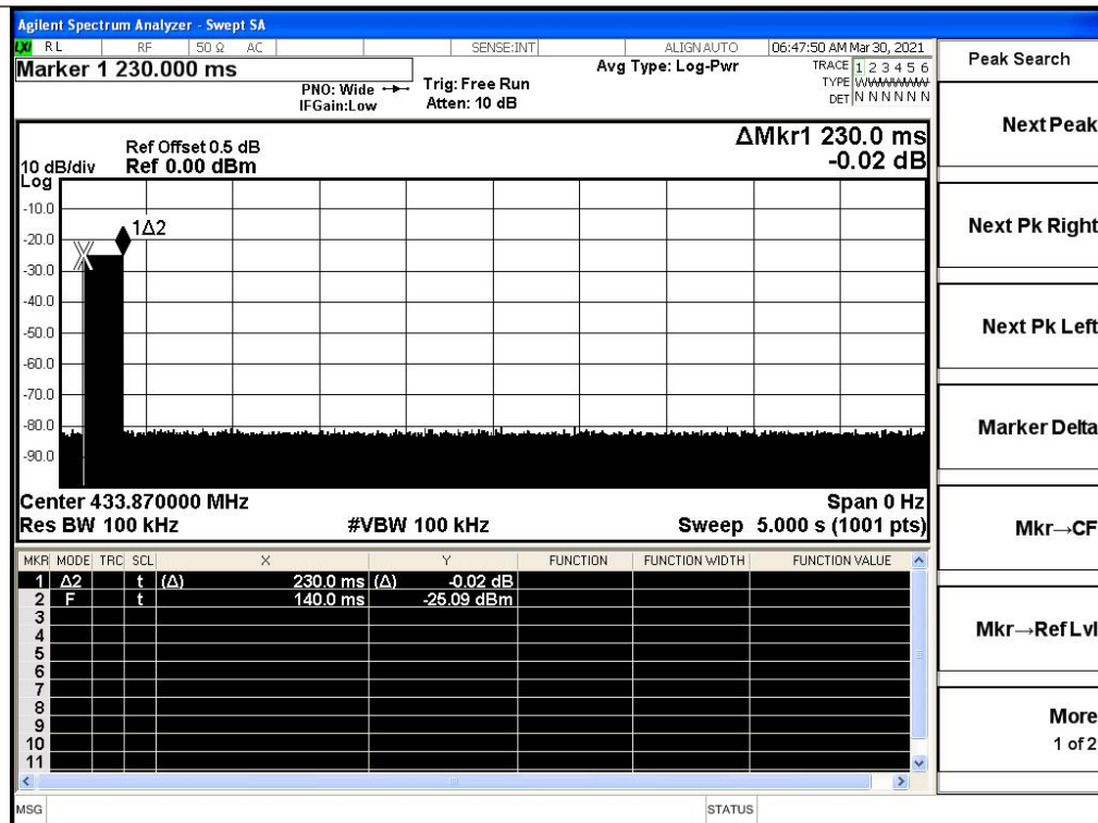
Fig.2:Pulse train is periodic with a period that exceeds 100 ms
