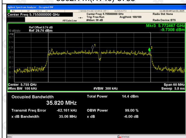
5802.11n(HT40)-5755
