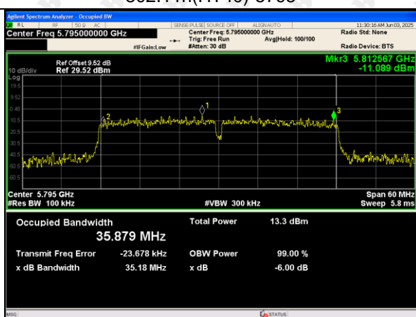
802.11n(HT40)-5795
