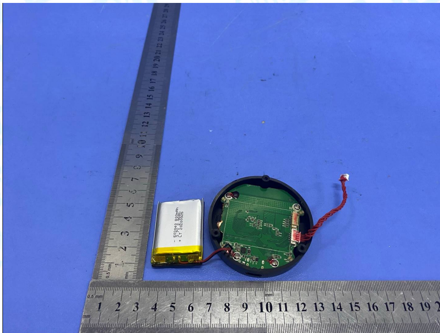
Photo 16 Internal of Battery
