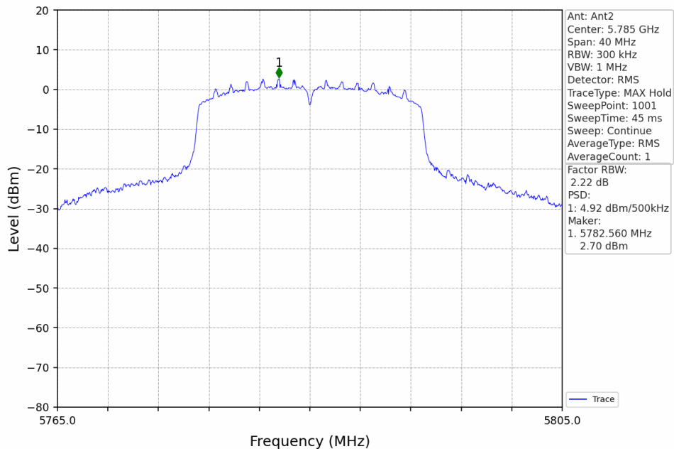
802.11n(HT20)_MCH_5785MHz_Ant2_NTNV
