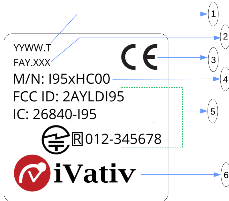
Figure 4: Module Label
