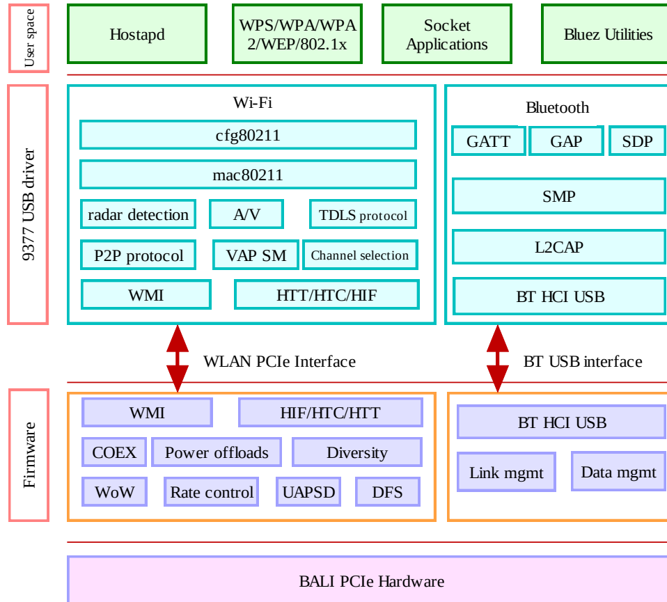
Figure 3: BALI PCIe Software Architecture
