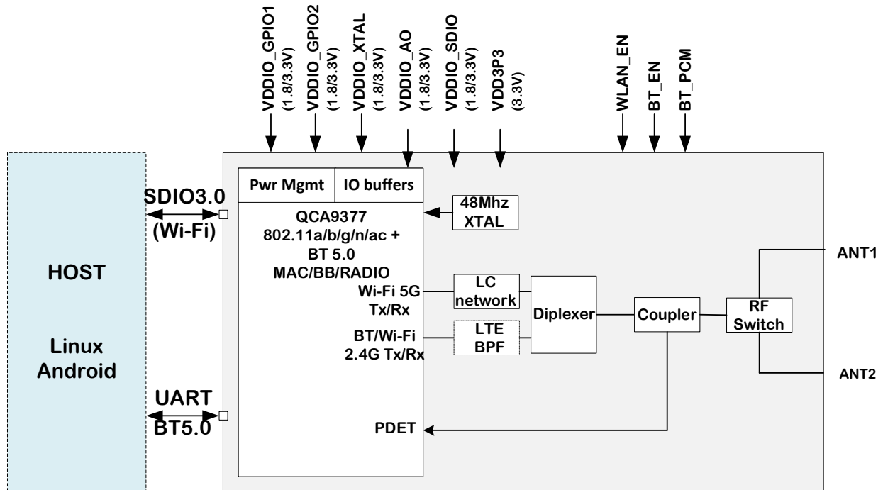
Figure 1: BALI block diagram
