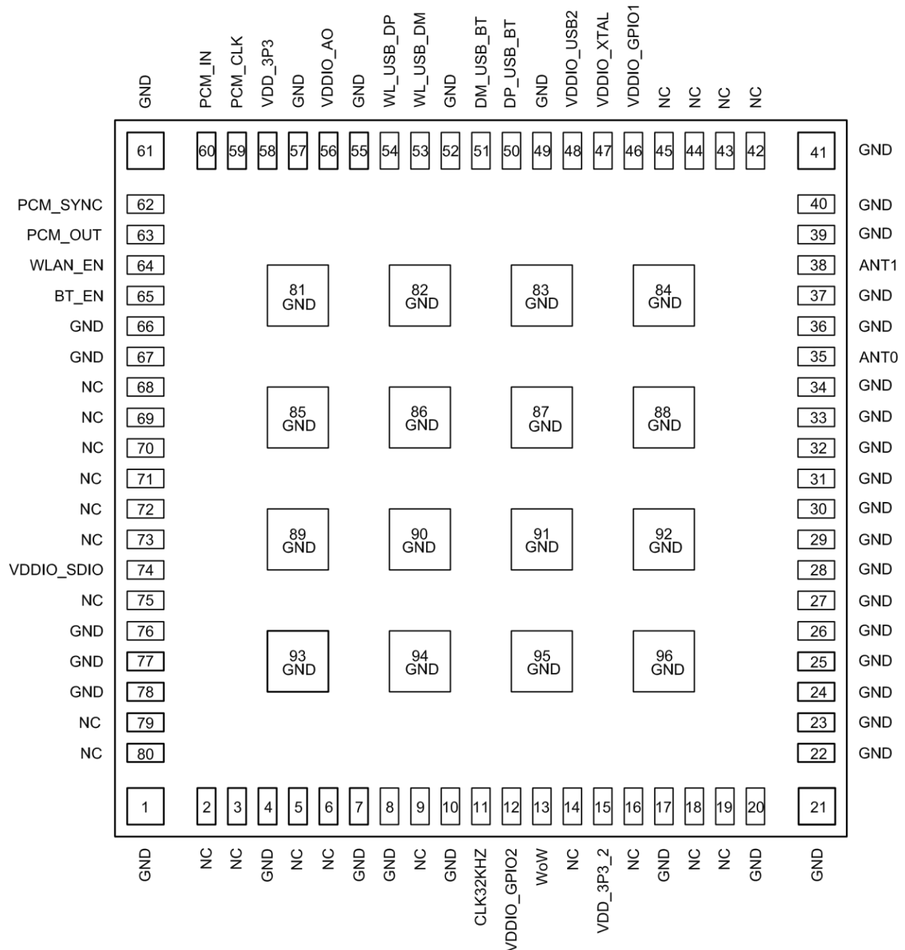
Figure 2: BALI Module Pin Diagram
