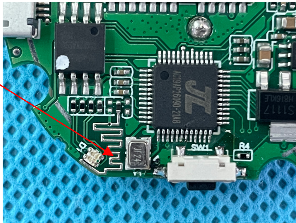
PCB Antenna
