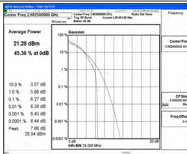
Band41-15MHz-16QAM-41515-75RB#0
