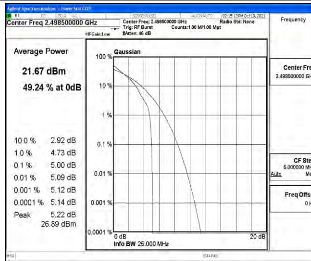
Band41-5MHz-QPSK-39675-25RB#0
