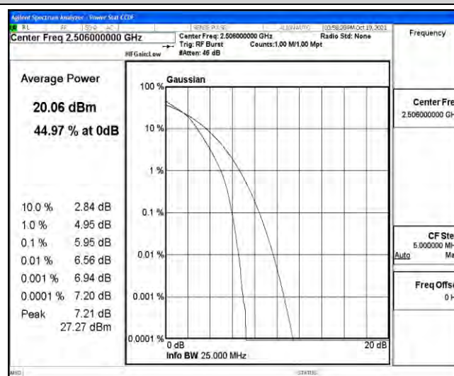
Band41-20MHz-16QAM-40620-1RB#0
