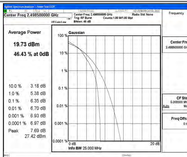
Band41-5MHz-16QAM-40620-1RB#0
