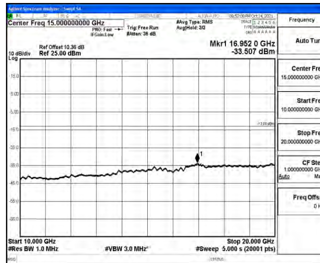
Band4-10MHz-16QAM-20000-1RB#0-Range1:0.009~0.15MHz
