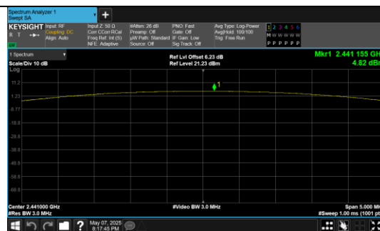
Peak Output Power GFSK_Channel 39
