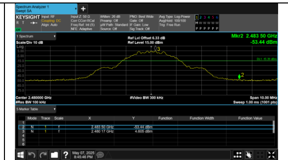
Out Of Band Emission \pi/4 DQPSK_2-DH5_Channel 78
