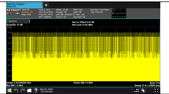
Number of Pulses in 31.6 seconds GFSK DH1
