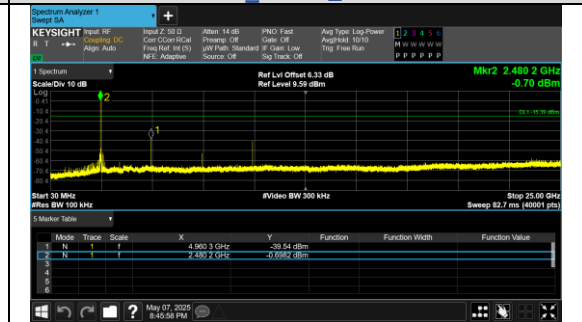
30.0 MHz - 25000.0 MHz \pi/4 DQPSK_2-DH5_Channel 78
