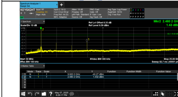
30.0 MHz - 25000.0 MHz GFSK_DH5_Channel 78
