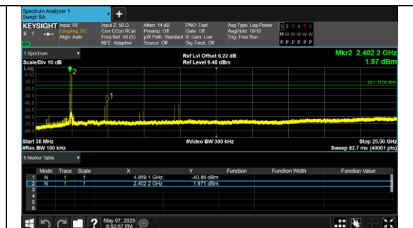
30.0 MHz - 25000.0 MHz 8DPSK_3-DH5_Channel 0
