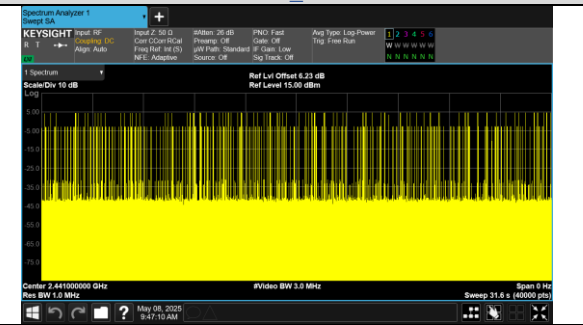
Number of Pulses in 31.6 seconds GFSK DH5
