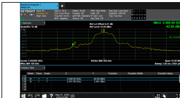
Out Of Band Emission 8DPSK_3-DH5_Channel 0
