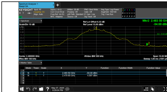
Out Of Band Emission GFSK_DH5_Channel 78
