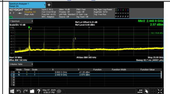
30.0 MHz - 25000.0 MHz 8DPSK_3-DH5_Channel 39
