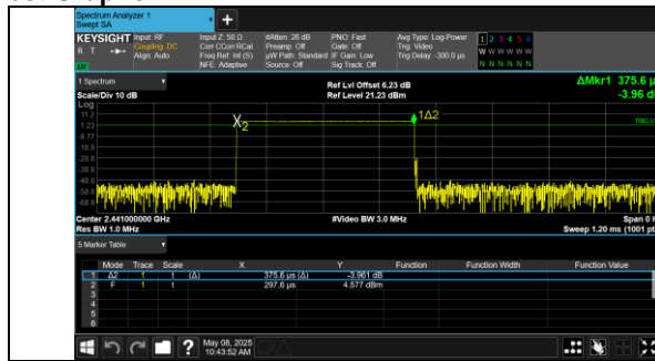
Pulse Width GFSK DH1
