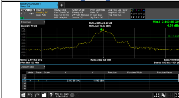
Out Of Band Emission 8DPSK_3-DH5_Channel 39
