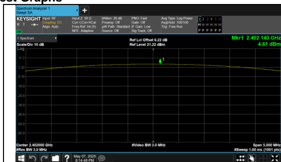
Peak Output Power GFSK_Channel 0
