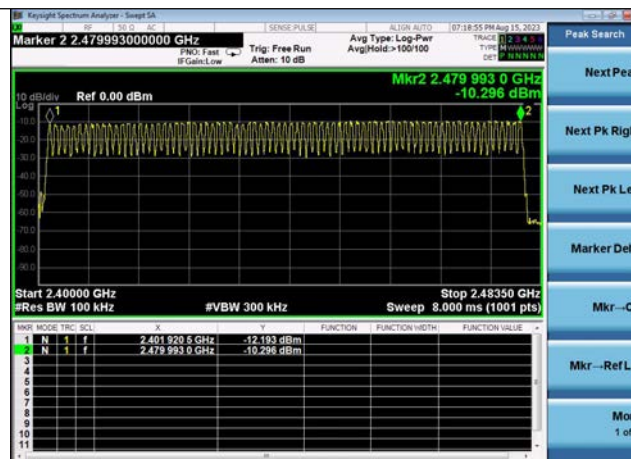
GFSK Modulation
