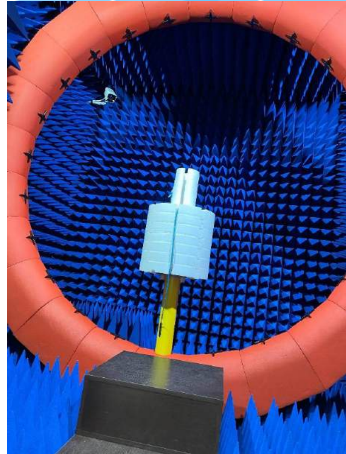
Microwave anechoic chamber FTM-24D multi-probe
