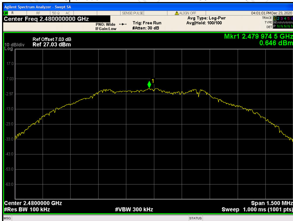
Tx. Spurious NVNT BLE 1M PHY 2480MHz Emission
