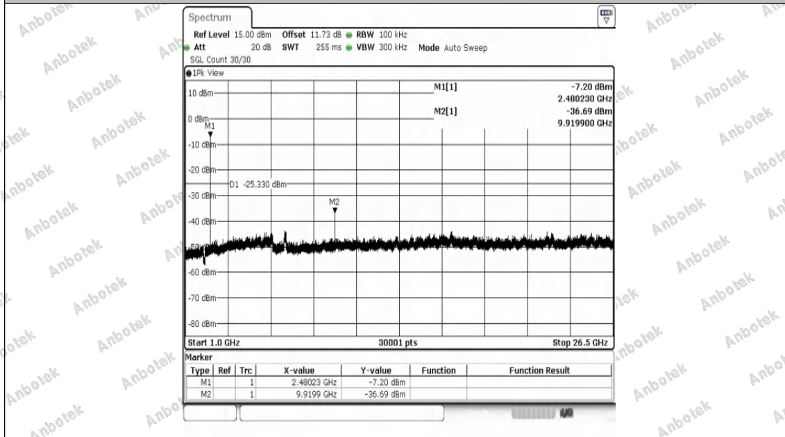
2DH5-Ant1-2480-1000~26500-PASS
