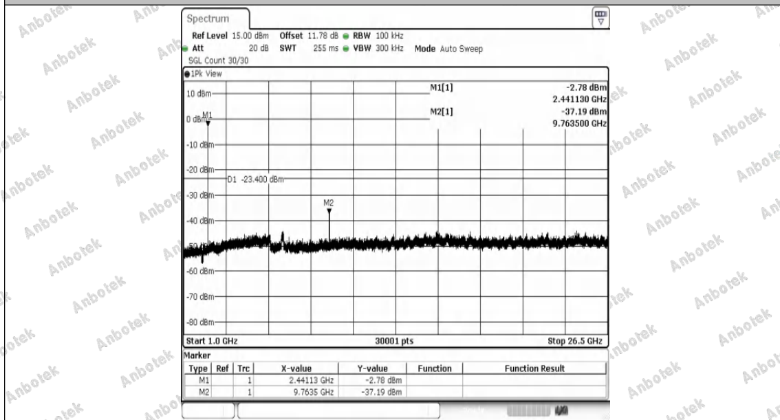
DH5-Ant1-2441-1000~26500-PASS
