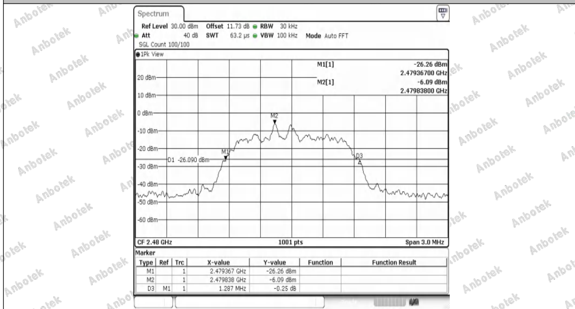
2DH5-Ant1-2480
