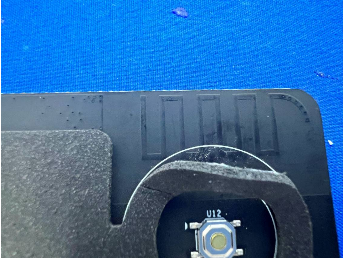
Lora Antenna(Rear View)
