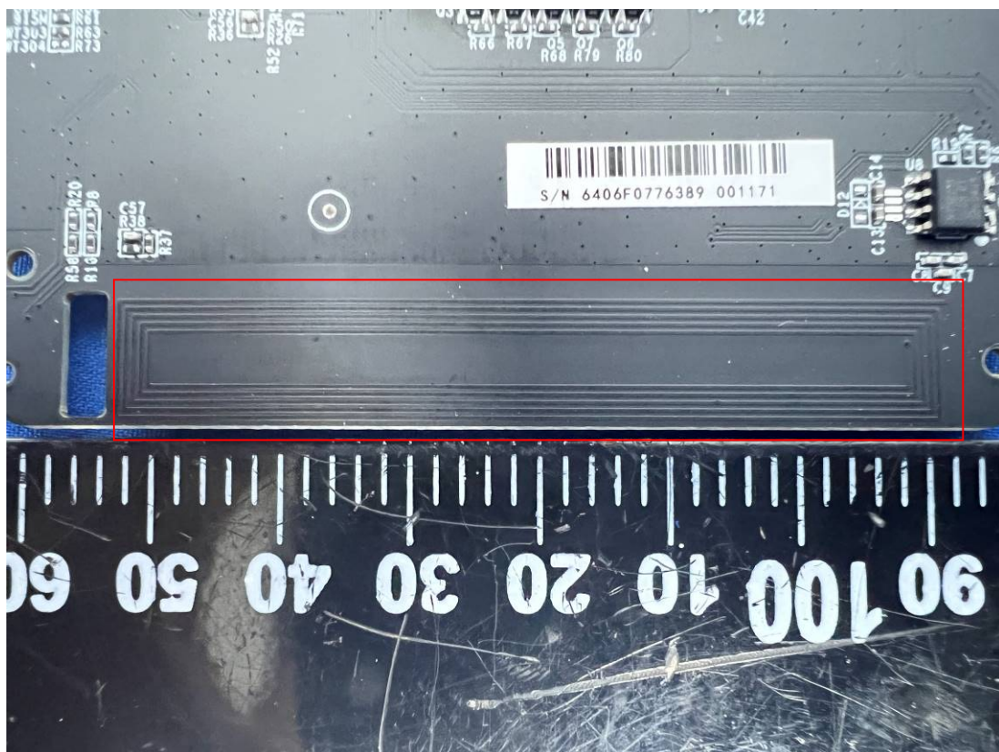
NFC Receiving Antenna
