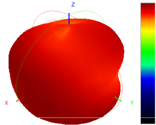
868.0MHz H+V, Eff: 7.2%
