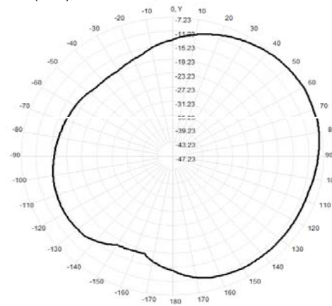
Total(H-XY), Max=-7.23dBi, CirD=11.71
