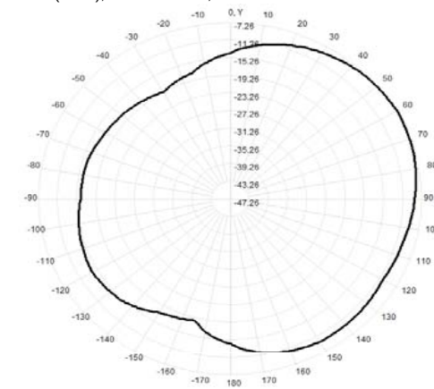
Total(H-XY), Max=-7.26dBi, CirD=12.04
