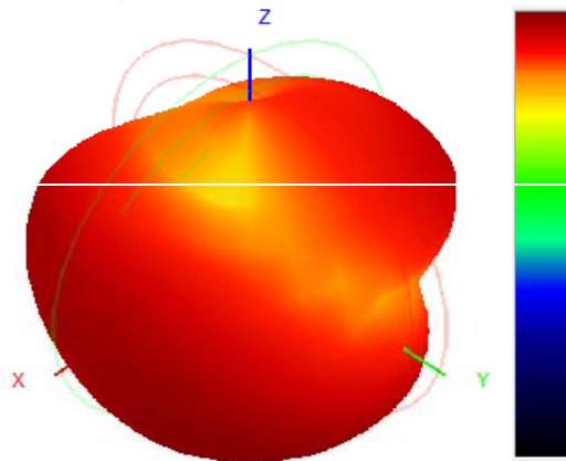
904.0MHz H+V, Eff: 6.6%
