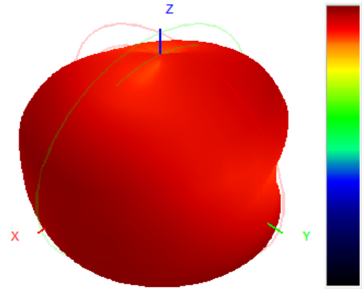
866.0MHz H+V, Eff: 7.1%
