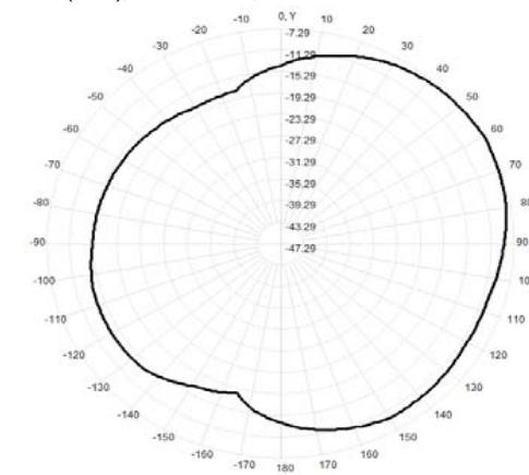
Total(H-XY), Max=-7.29dBi, CirD=11.39
