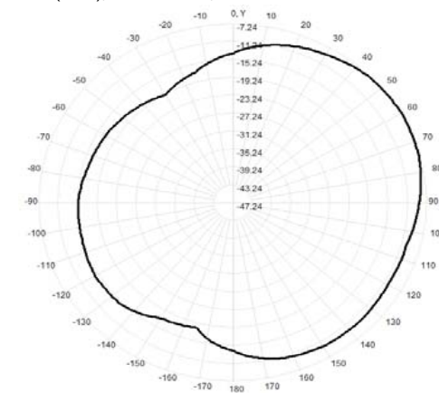
Total(H-XY), Max=-7.24dBi, CirD=12.22
