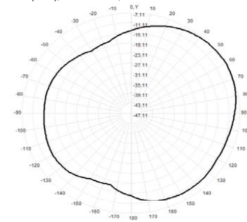
Total(H-XY), Max=-7.11dBi, CirD=11.27
