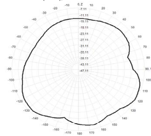
929.0MHz Total(E2-YZ), Max=-7.82dBi
