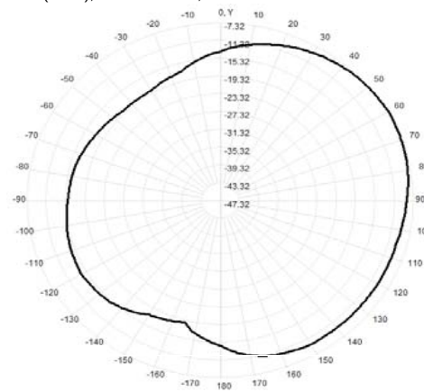
Total(H-XY), Max=-7.32dBi, CirD=11.66
