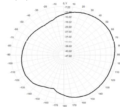
Total(H-XY), Max=-7.22dBi, CirD=11.66
