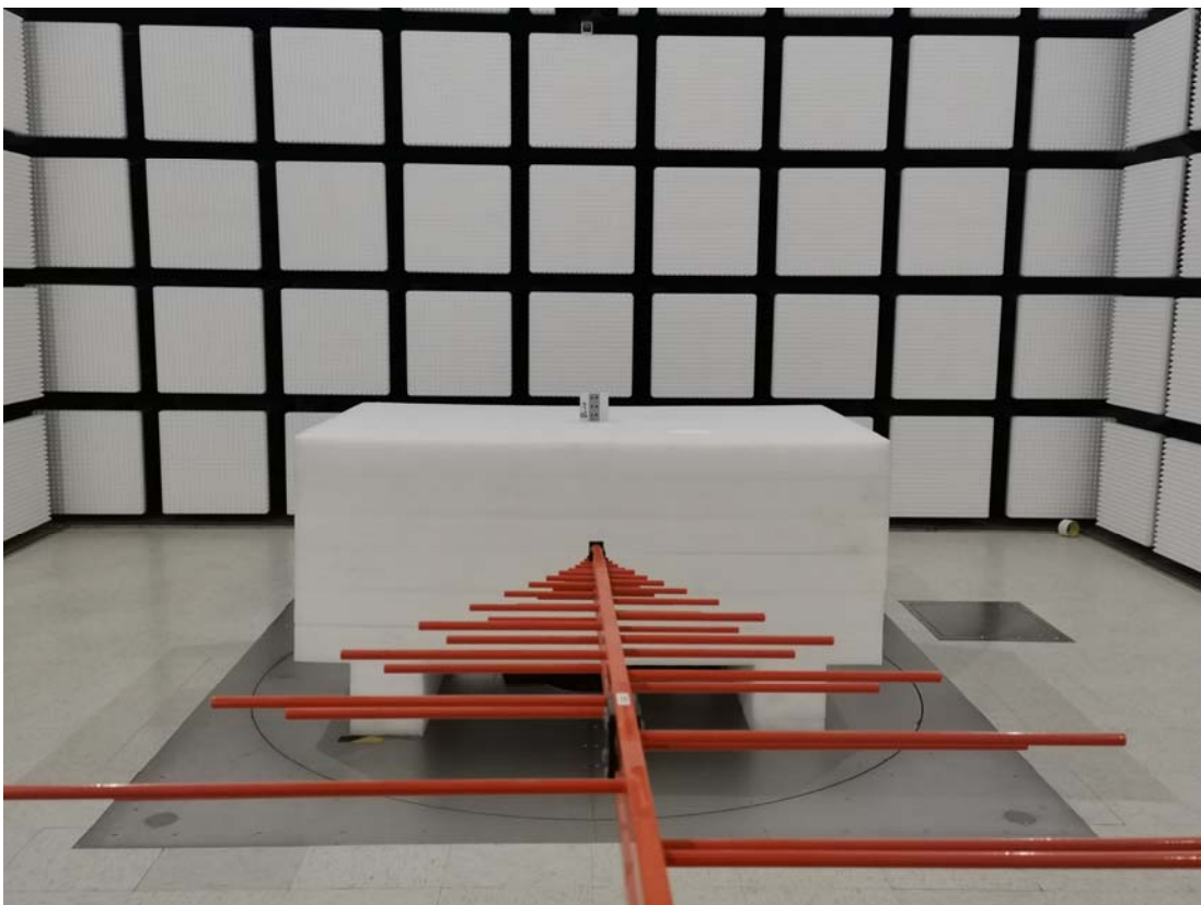
Radiated Emission Below 1GHz View- WS136-915M
