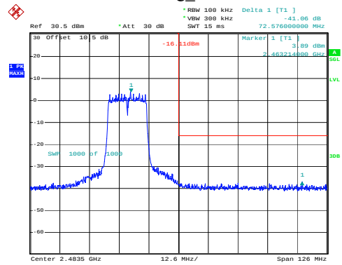
802.11g_2462MHz
