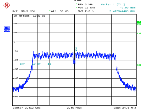
802.11g_2412MHz
