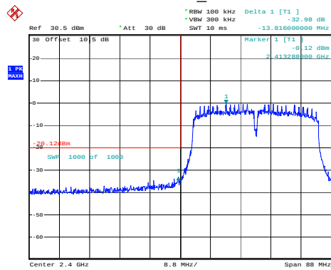
802.11n40_2422MHz
