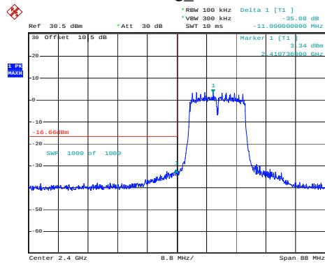
802.11g_2412MHz
