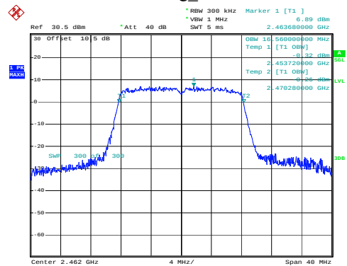
802.11g_2462MHz
