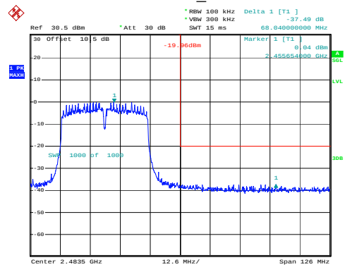
802.11n40_2452MHz
