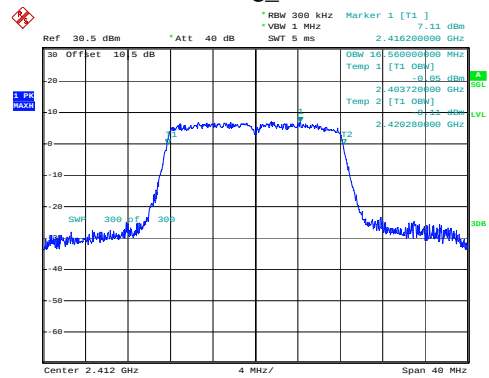
802.11g_2412MHz
