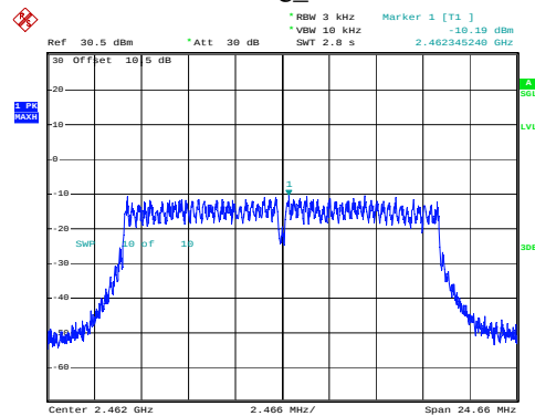
802.11g_2462MHz
