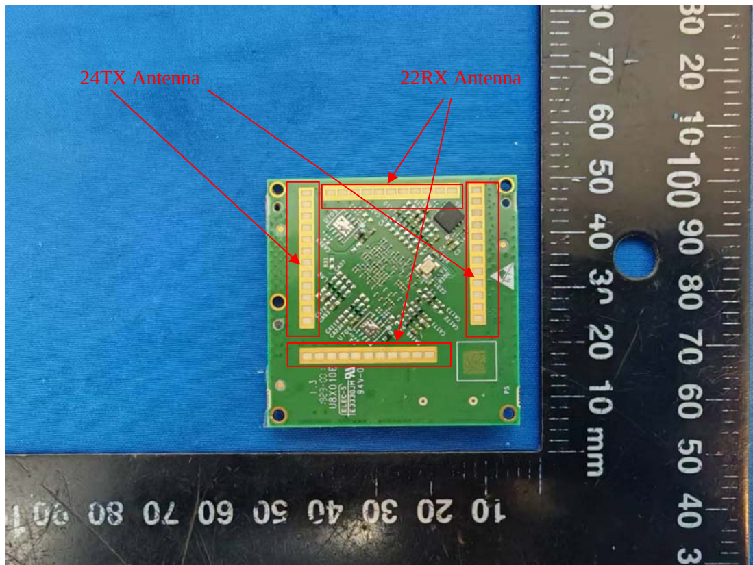
60G Radar Chip
