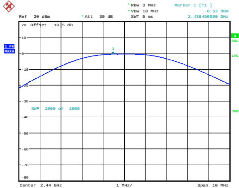
BLE_2M_Middle_Channel
