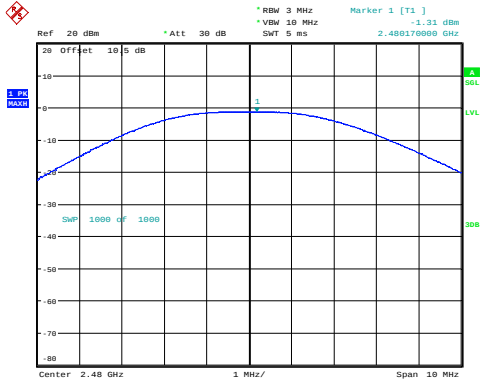
BLE_2M_High_Channel
