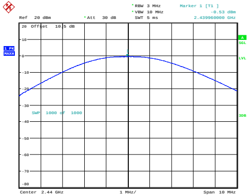
BLE_1M_Middle_Channel
