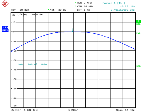
BLE_2M_Low_Channel
