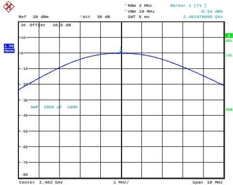
BLE_1M_Low_Channel
