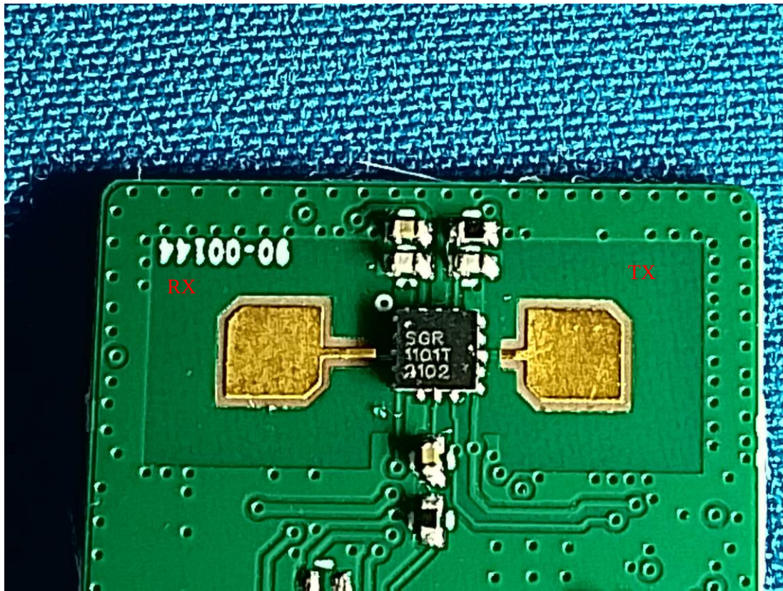
Radar Chip+Antenna
