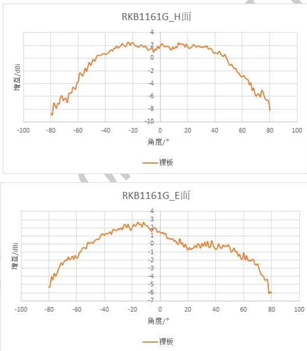
Antenna Radiation Pattern Measurement Data
