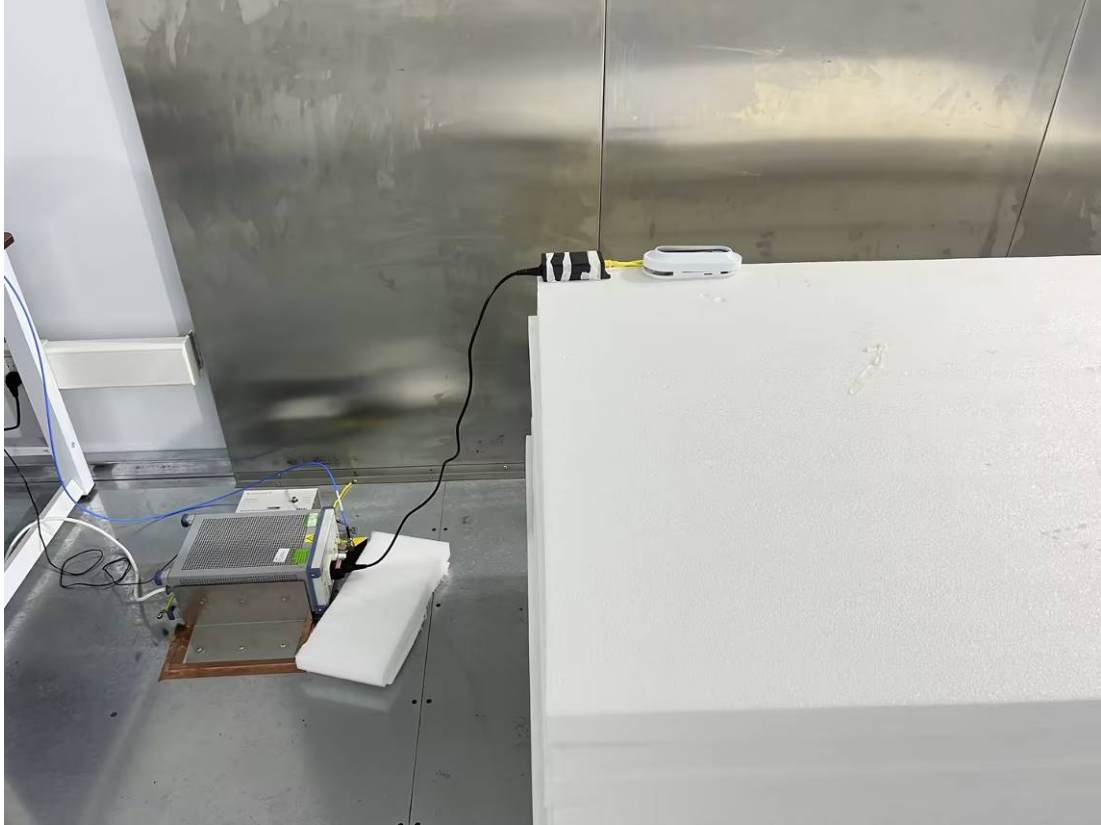
CE- Side View (PoE)
