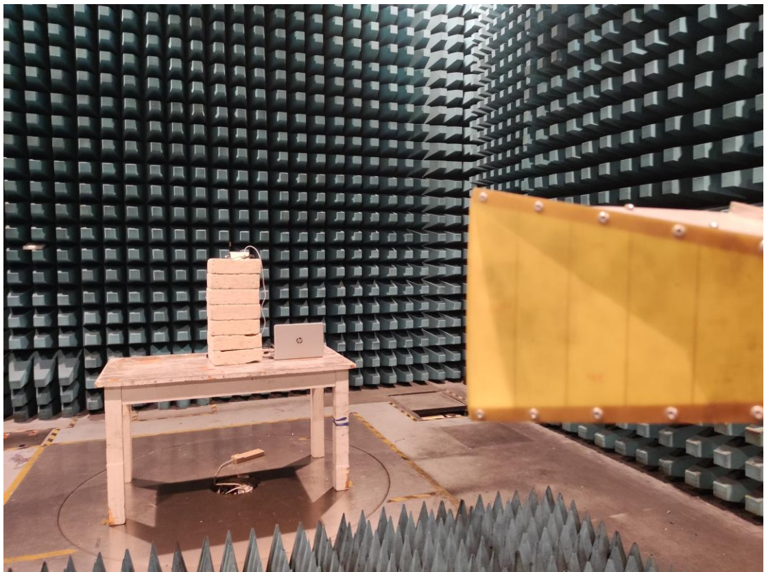
RSE_ Above 1 GHz_External Ant(long)
