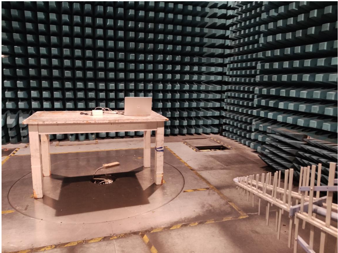
RSE_ from 30 MHz to 1 GHz_External Ant(long)
