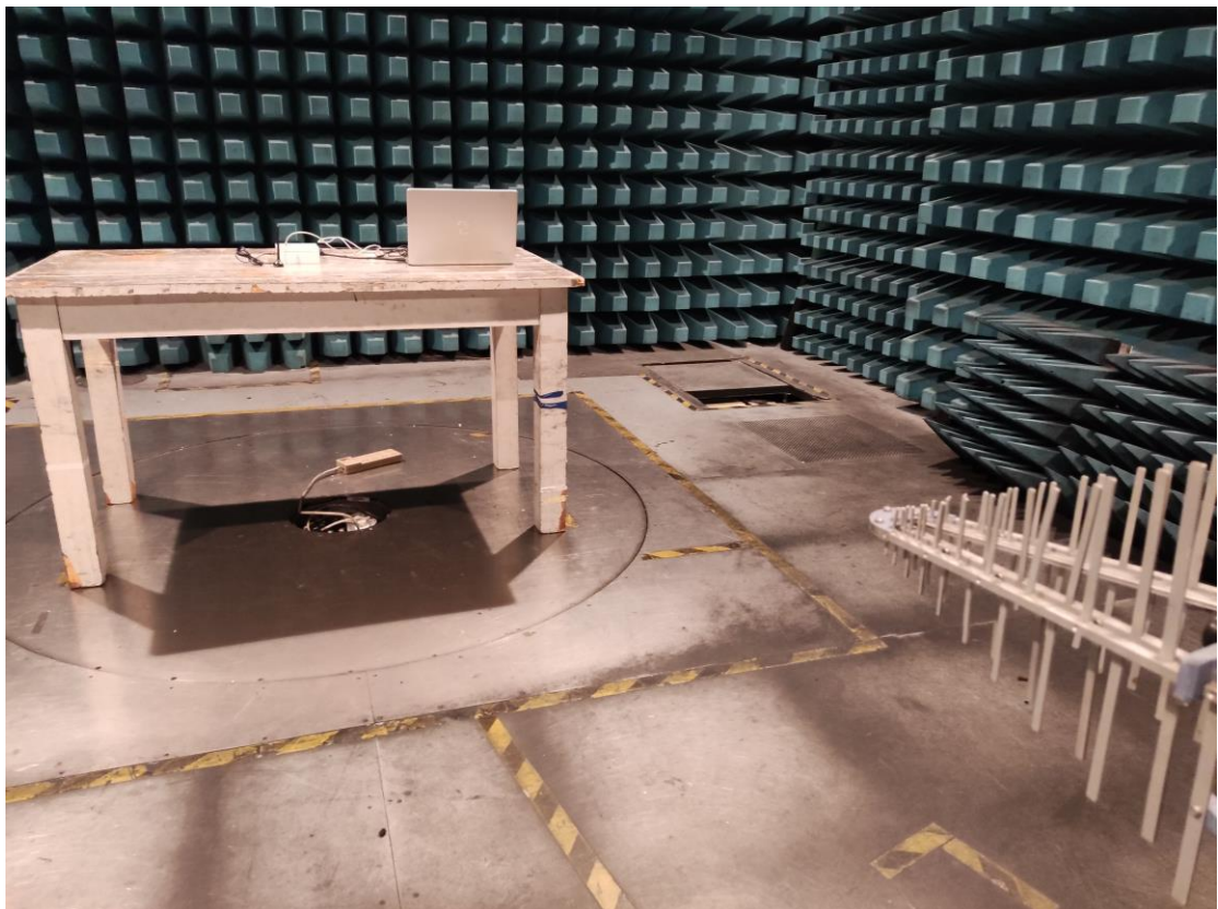
RSE_ from 30 MHz to 1 GHz_External Ant(short)
