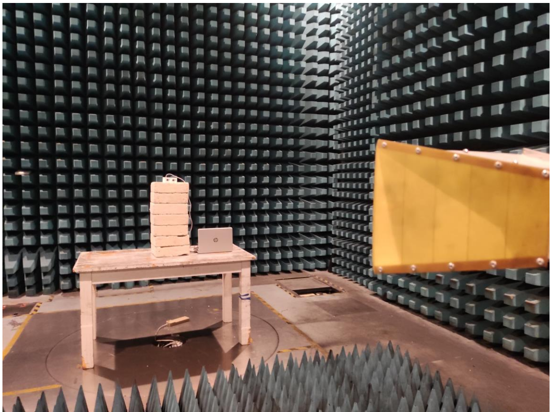
RSE_ Above 1 GHz_Internal Ant
