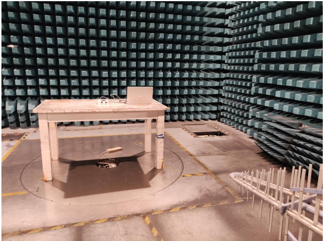
RSE_ from 30 MHz to 1 GHz_Internal Ant
