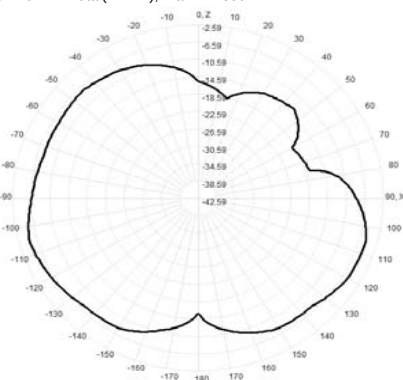
914.0MHz Total(E1-XZ), Max= -4.89dBi
