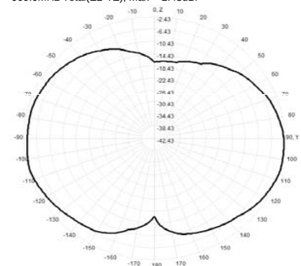
909.0MHz Total(E2-YZ), Max= -2.43dBi
