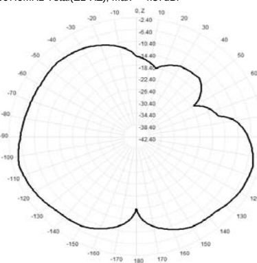
907.0MHz Total(E1-XZ), Max= -4.37dBi
