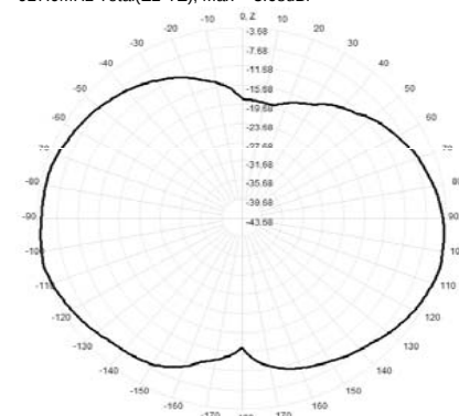
927.0MHz Total(E2-YZ), Max= -3.68dBi
