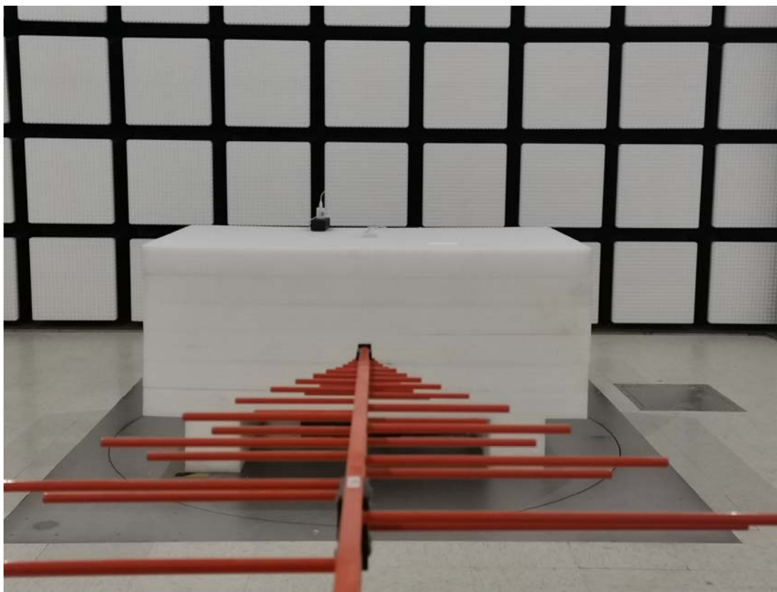
DC power mode: Radiated Emission Below 1GHz View
