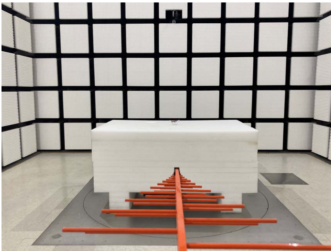
DC power mode: Radiated Emission Below 1GHz View
