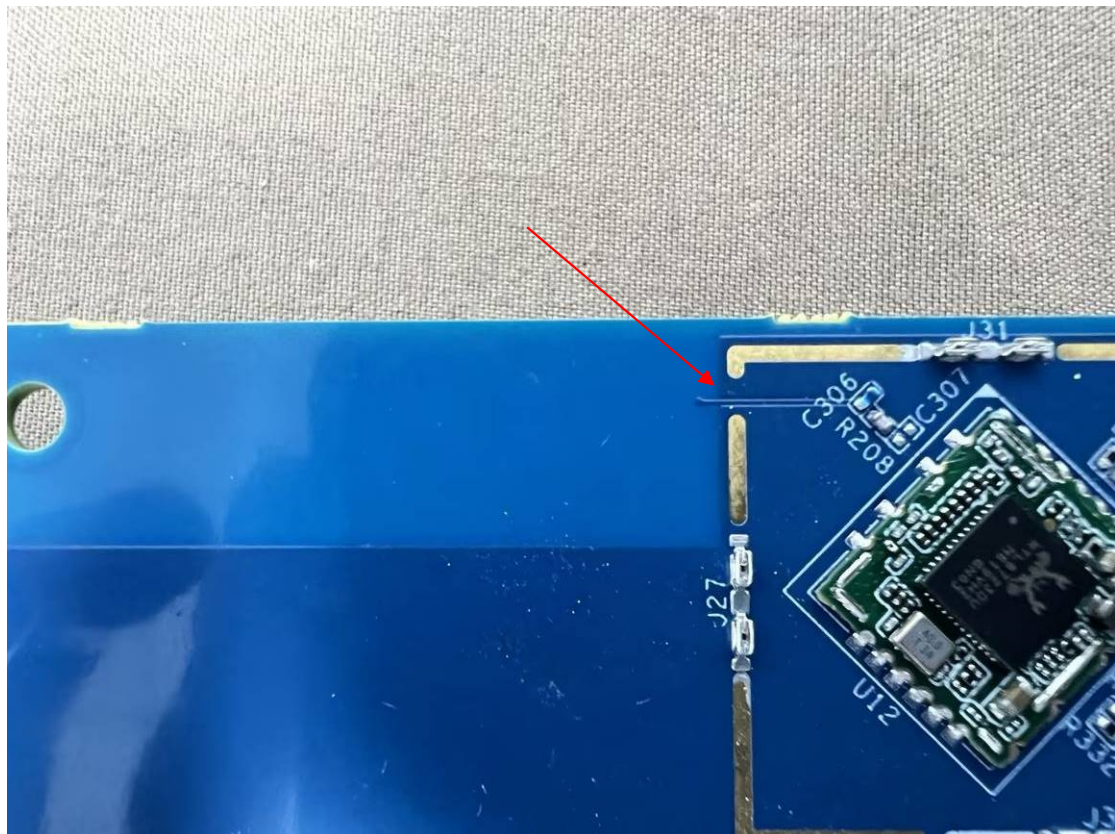
WIFI Antenna-Front Side View
