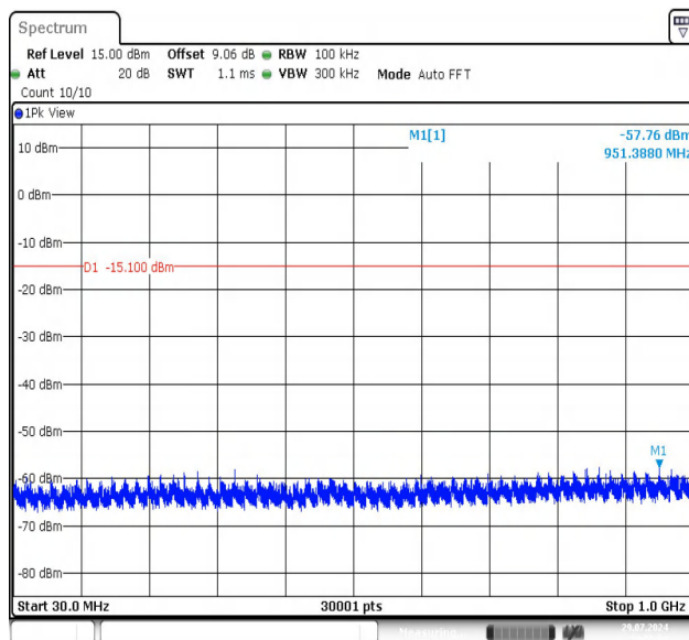
BLE_1M-Ant1-2480-30~1000-PASS
