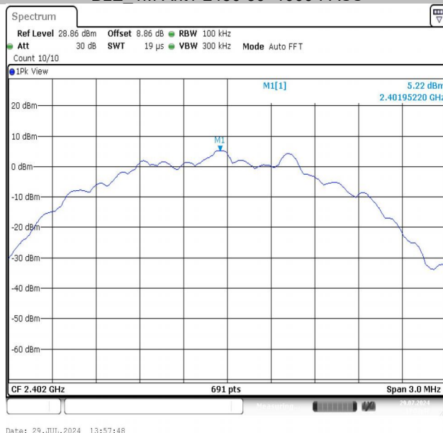
BLE_2M-Ant1-2402-0~Reference-PASS
