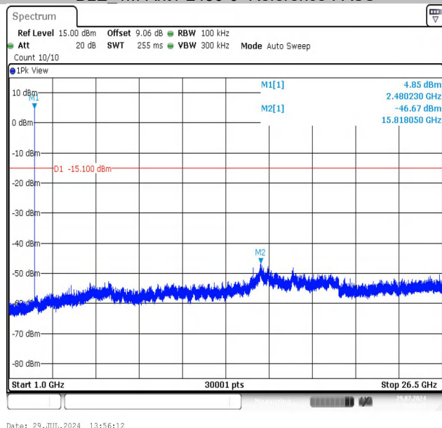
BLE_1M-Ant1-2480-1000~26500-PASS
