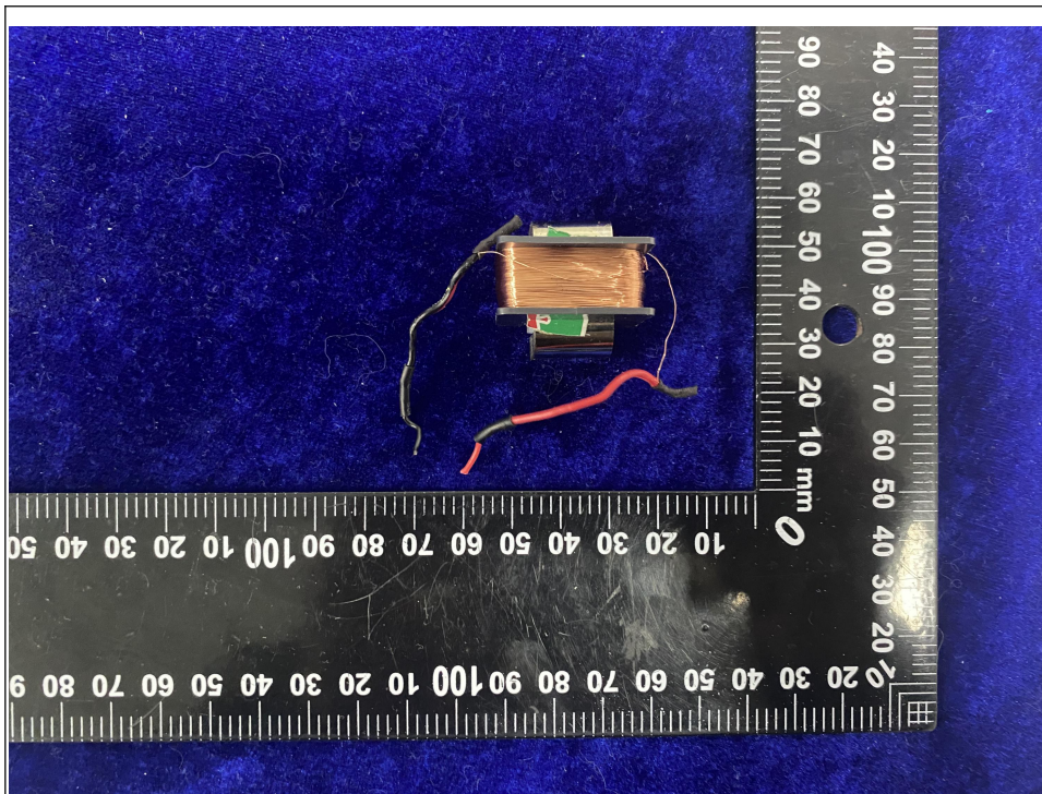
300A Transformer
