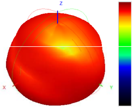
909.0MHz H+V, Eff: 2.1%
