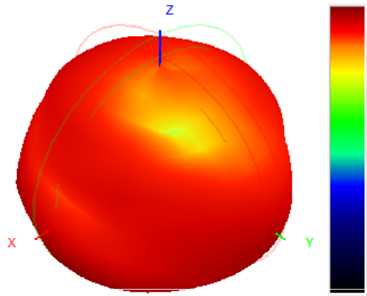
910.0MHz H+V, Eff: 2.2%
