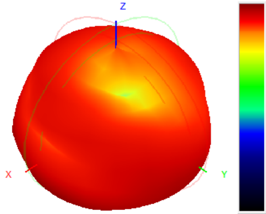
908.0MHz H+V, Eff: 2.1%
