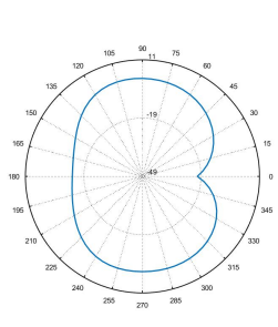
Total_Polar_E1_5.15GHz
