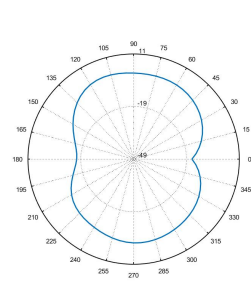
Total_Polar_E2_5.15GHz
