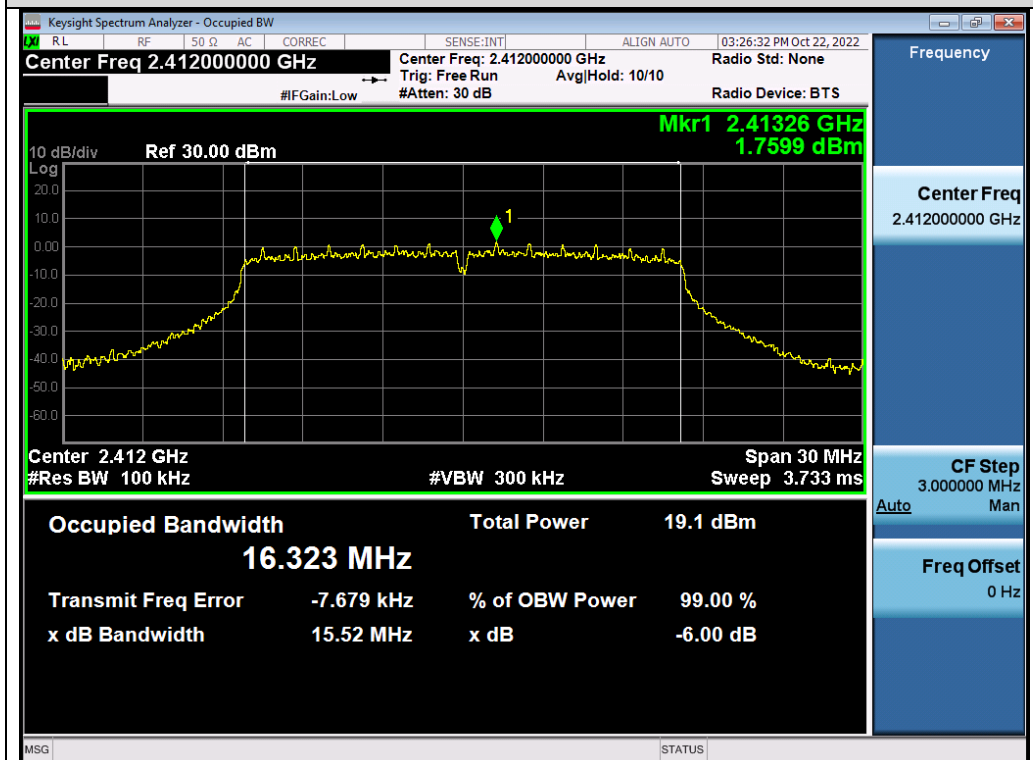
Test_Graph_802.11g_ANT2_2412_6Mbps_DTSBW
