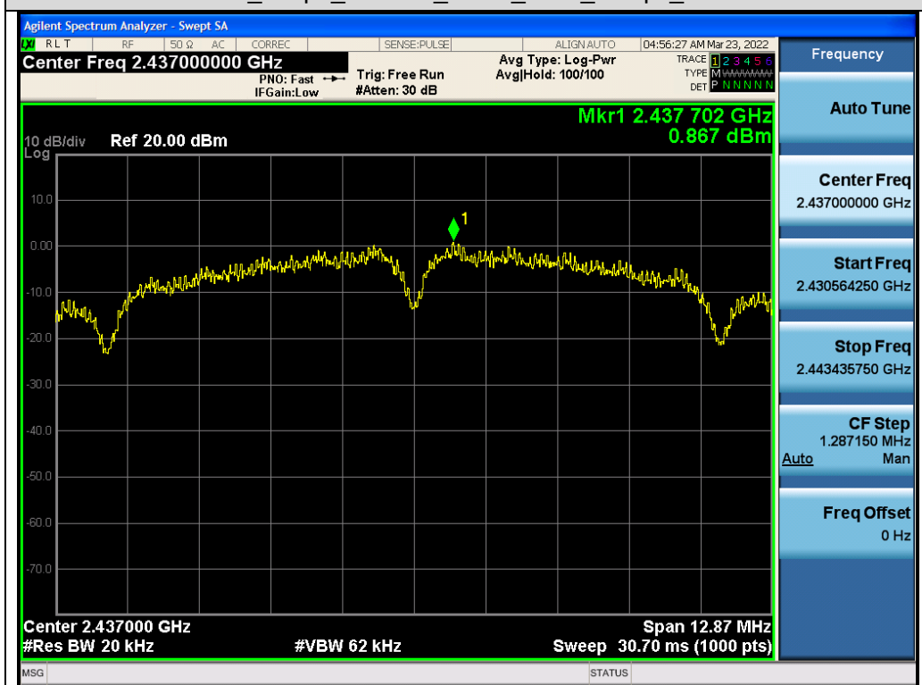
Test_Graph_802.11b_ANT1_2437_1Mbps_PSD
