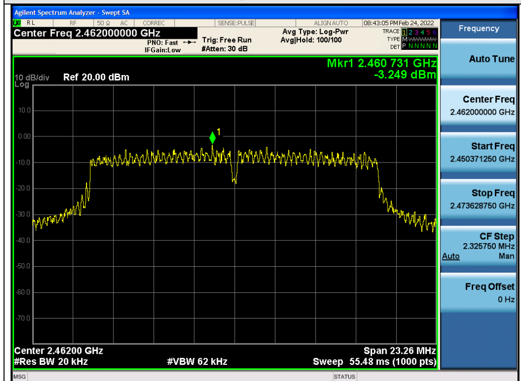
Test_Graph_802.11g_ANT2_2462_6Mbps_PSD
