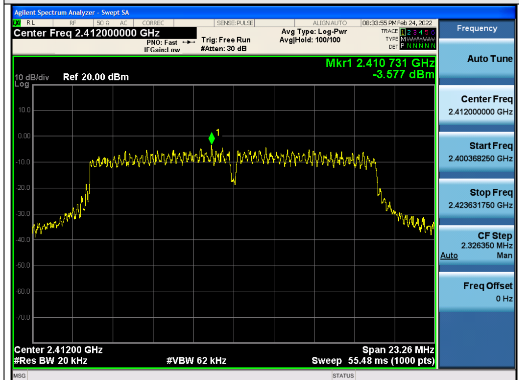
Test_Graph_802.11g_ANT2_2412_6Mbps_PSD
