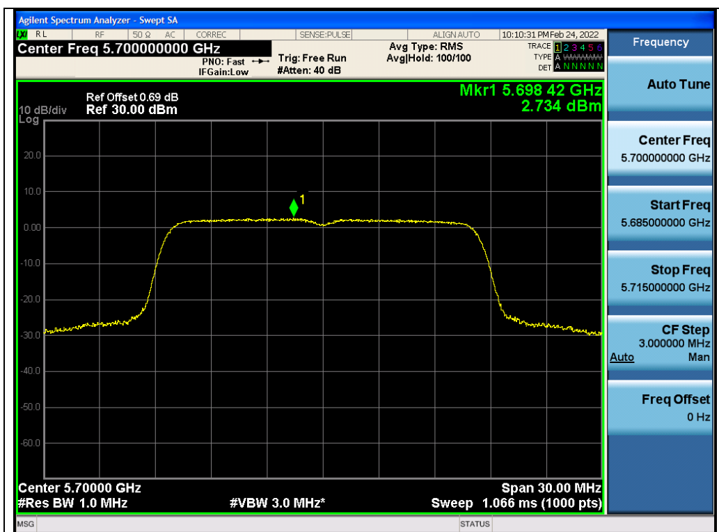
Test_Graph_802.11a_ANT1_5700_6Mbps_PSD
