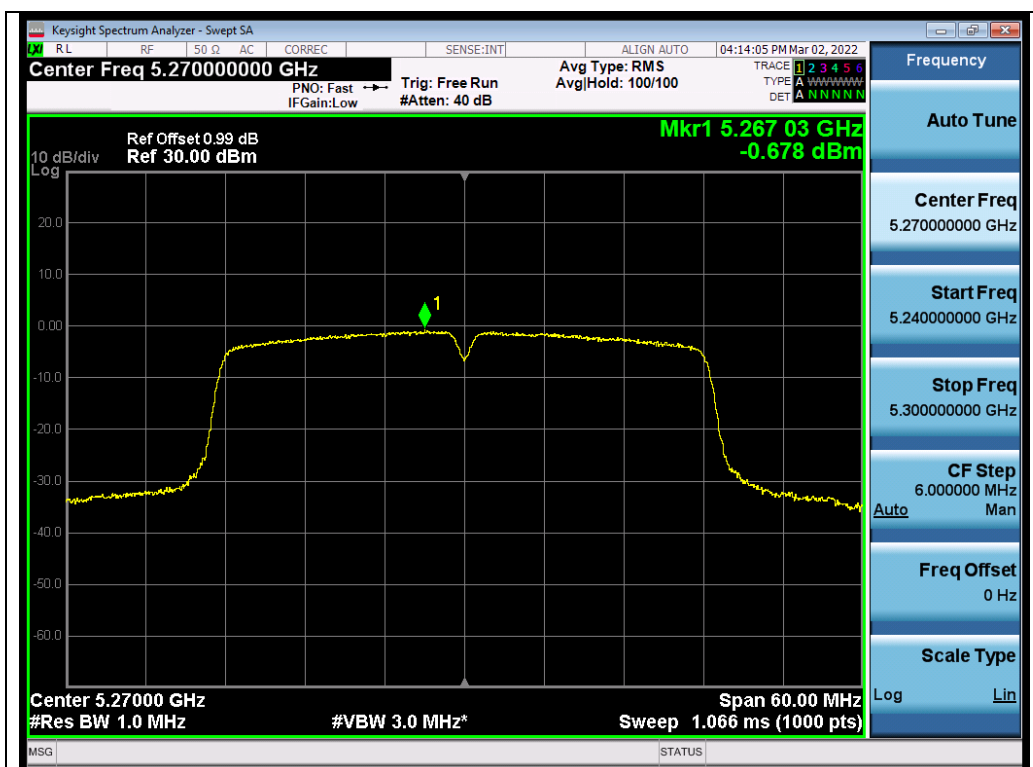
Test_Graph_802.11n40_ANT2_5270_MCS0_PSD
