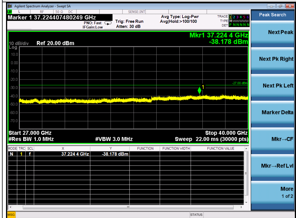
Test_Graph_802.11n40_ANT1_5590_MCS0_Frequency Band 5
