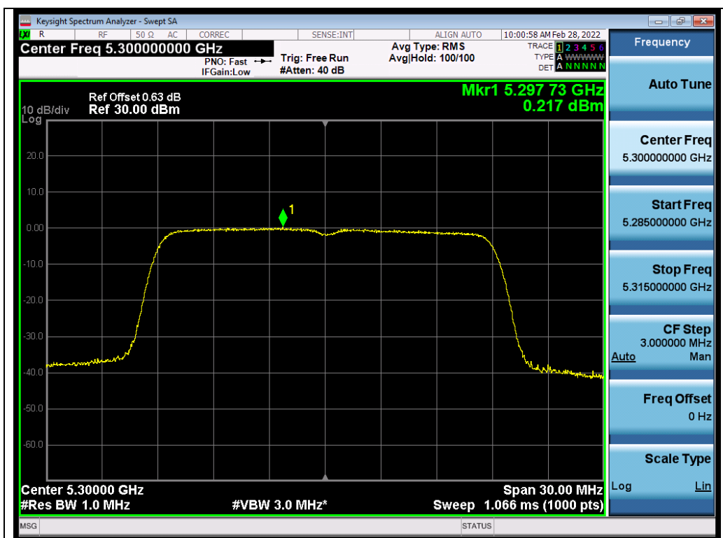
Test_Graph_802.11n20_ANT2_5300_MCS0_PSD
