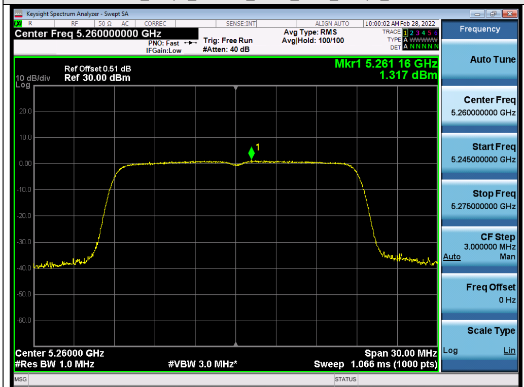
Test_Graph_802.11n20_ANT2_5260_MCS0_PSD
