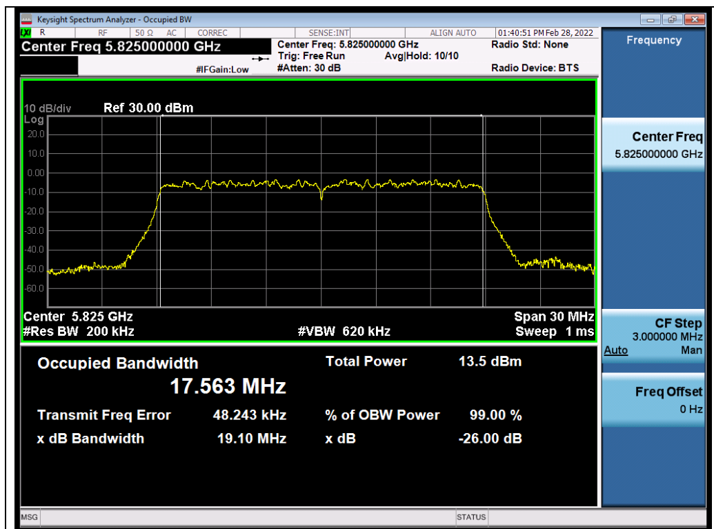
Test_Graph_802.11ac20_ANT2_5825_MCS9_OBW
