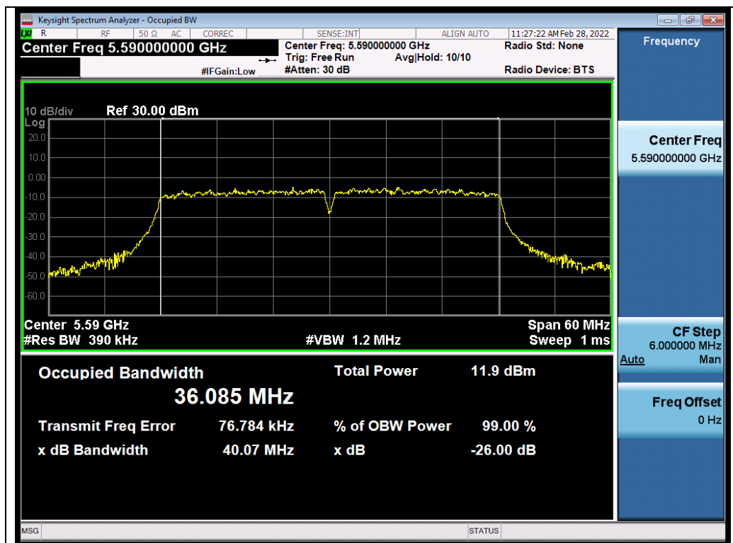
Test_Graph_802.11ac40_ANT2_5590_MCS9_OBW
