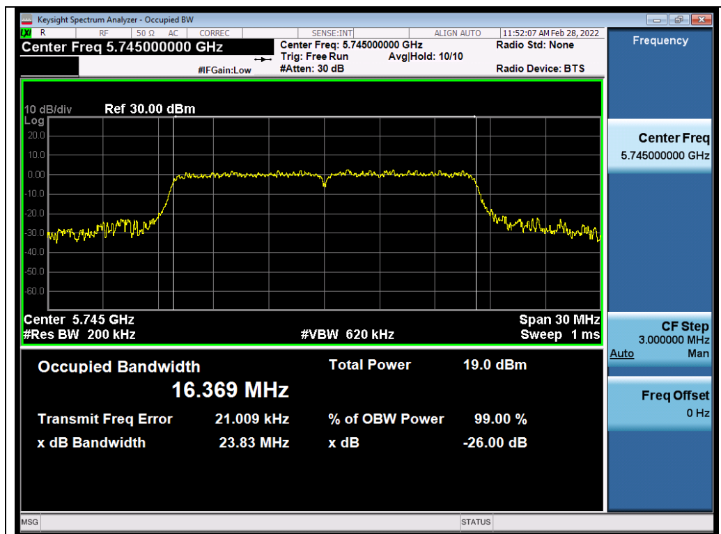
Test_Graph_802.11a_ANT2_5745_6Mbps_OBW
