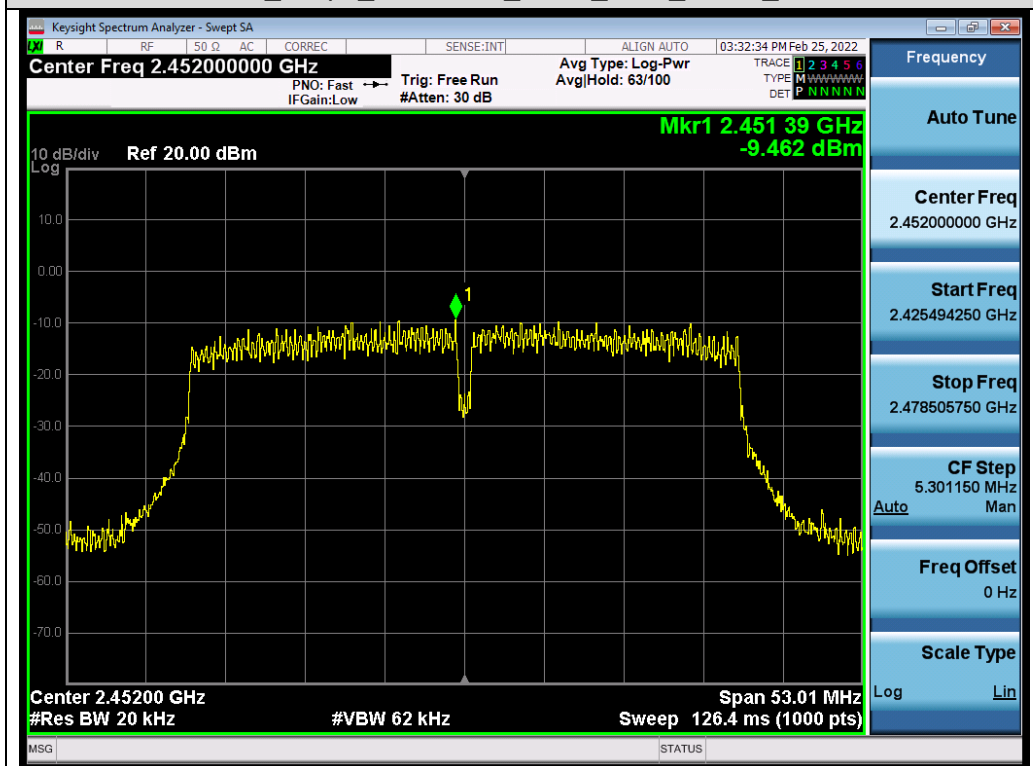
Test_Graph_802.11n40_ANT2_2452_MCS0_PSD
