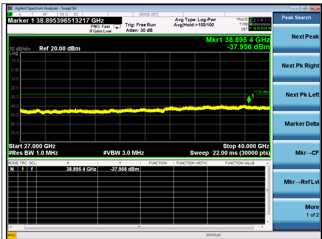
Test_Graph_802.11n40_ANT1_5670_MCS0_Frequency Band 5
