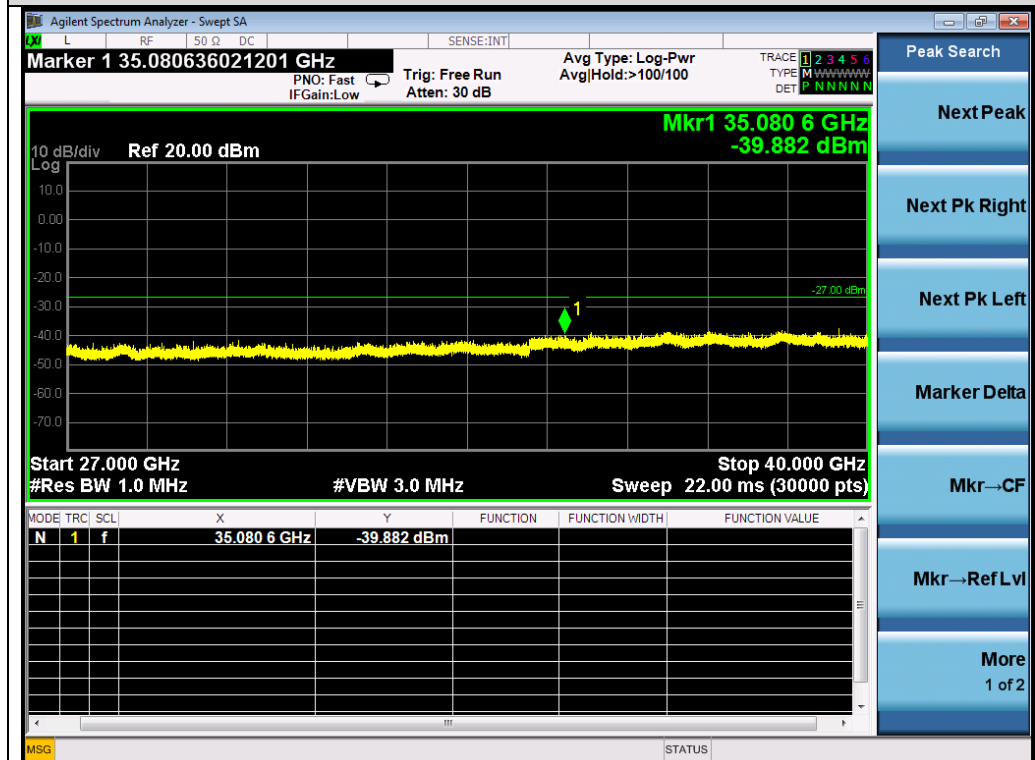
Test_Graph_802.11a_ANT1_5320_6Mbps_Frequency Band 5
