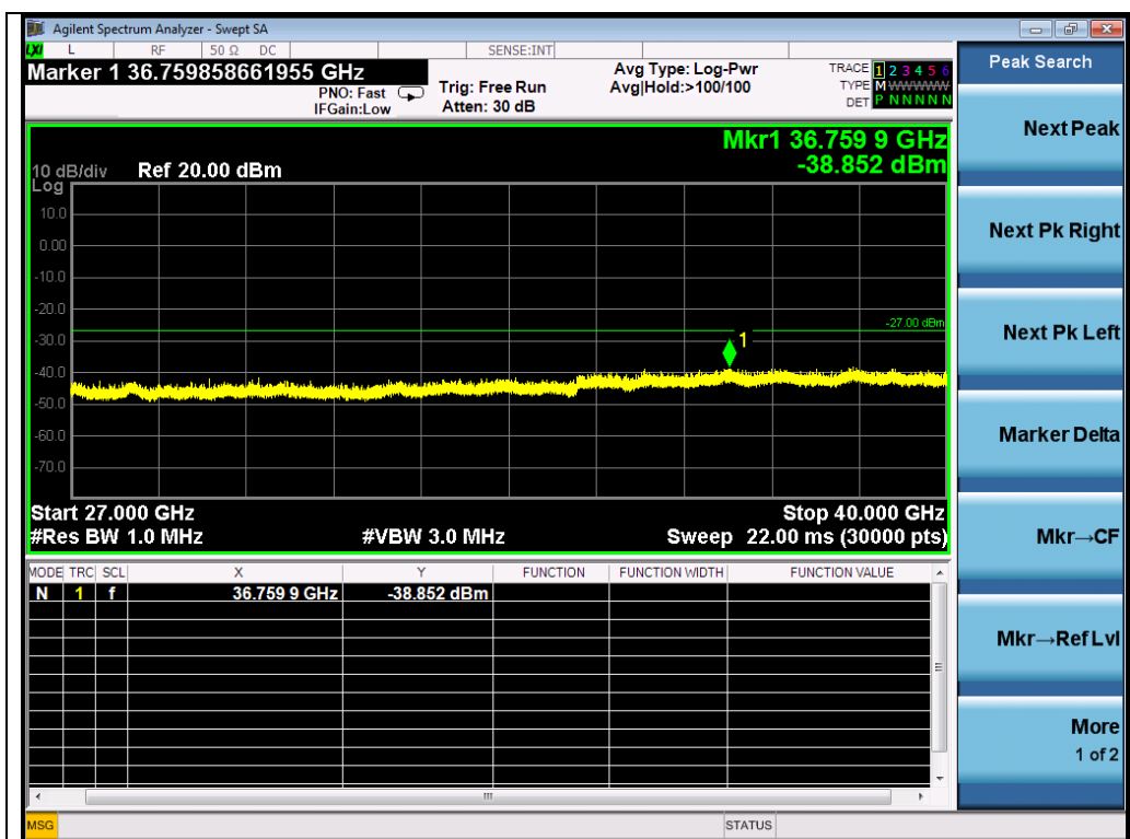
Test_Graph_802.11a_ANT1_5260_6Mbps_Frequency Band 5
