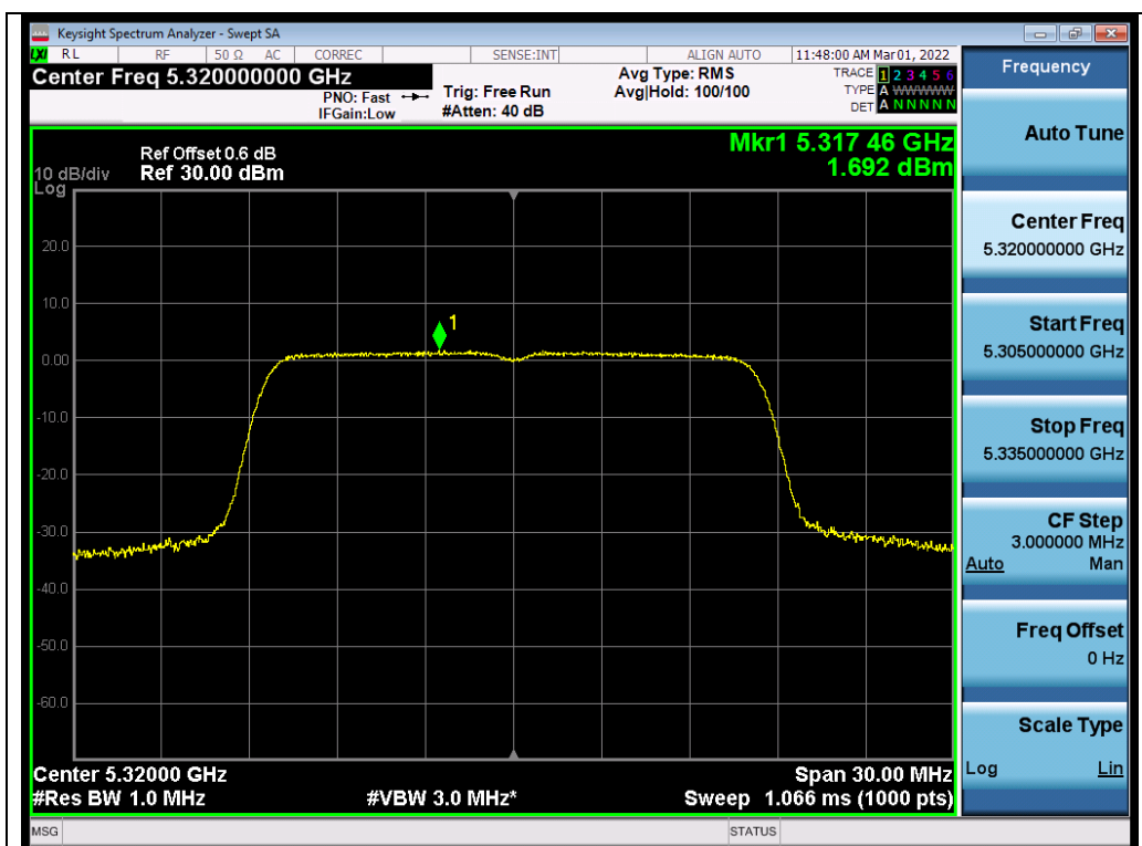
Test_Graph_802.11a_ANT2_5320_6Mbps_PSD
