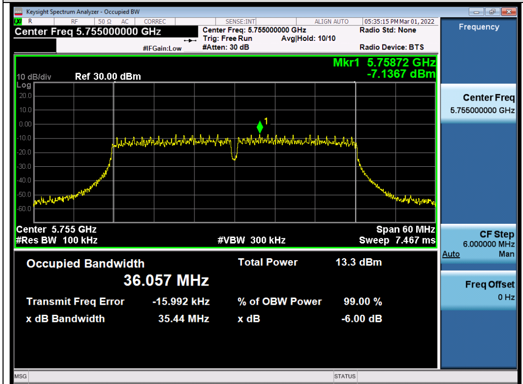
Test_Graph_802.11ac40_ANT1_5755_MCS9_DTSBW
