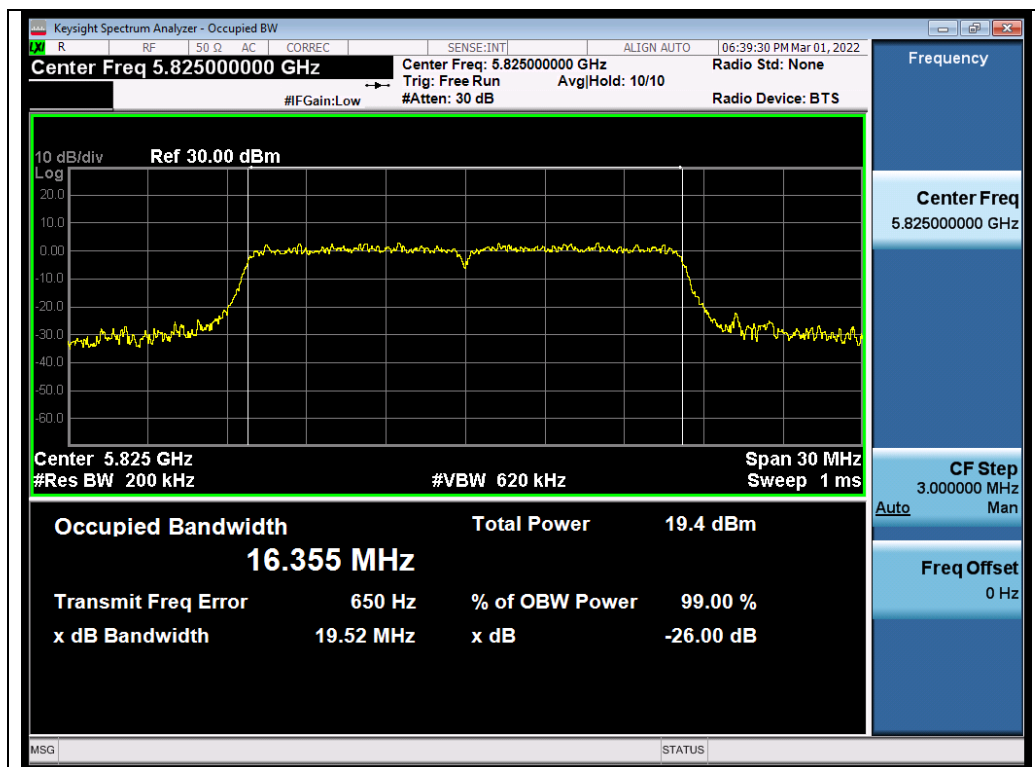
Test_Graph_802.11a_ANT2_5825_6Mbps_OBW
