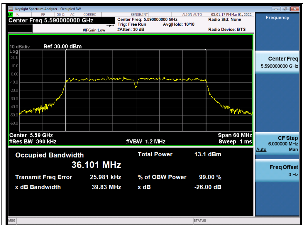
Test_Graph_802.11ac40_ANT2_5590_MCS9_OBW
