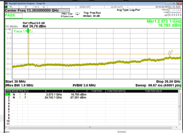
Band38_5M_16QAM_Middle
