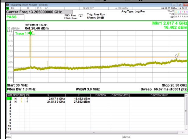
Band38_5M_QPSK_High
