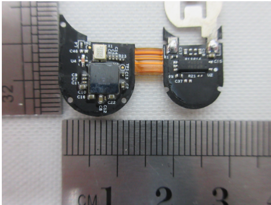
Main board_Rear
