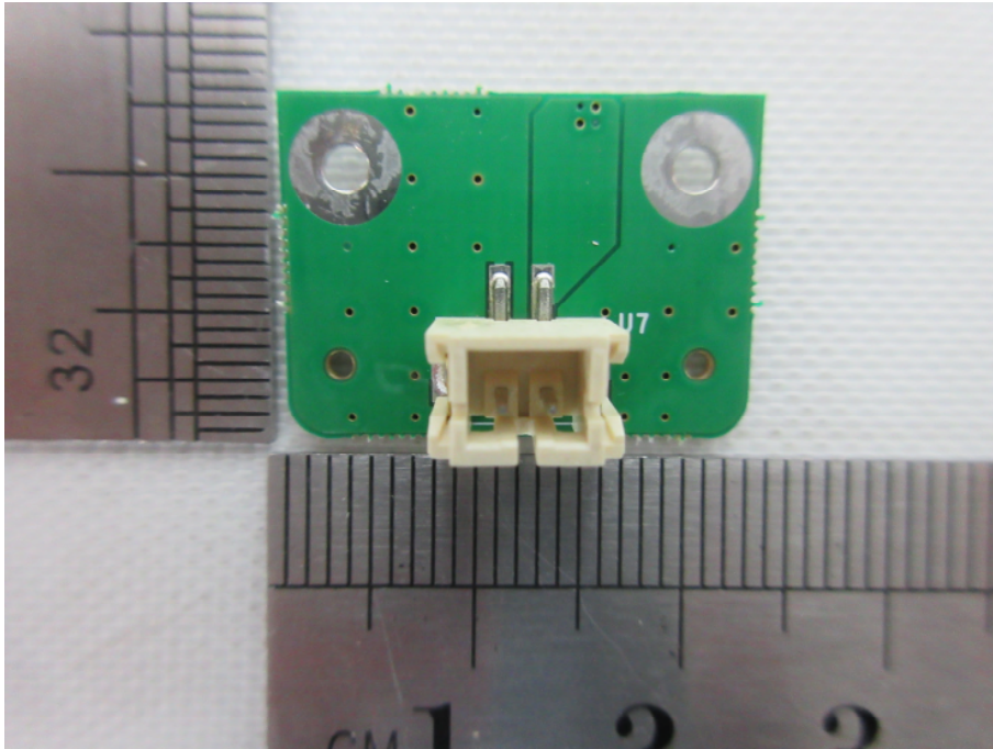
Cradle_Sub board_Front
