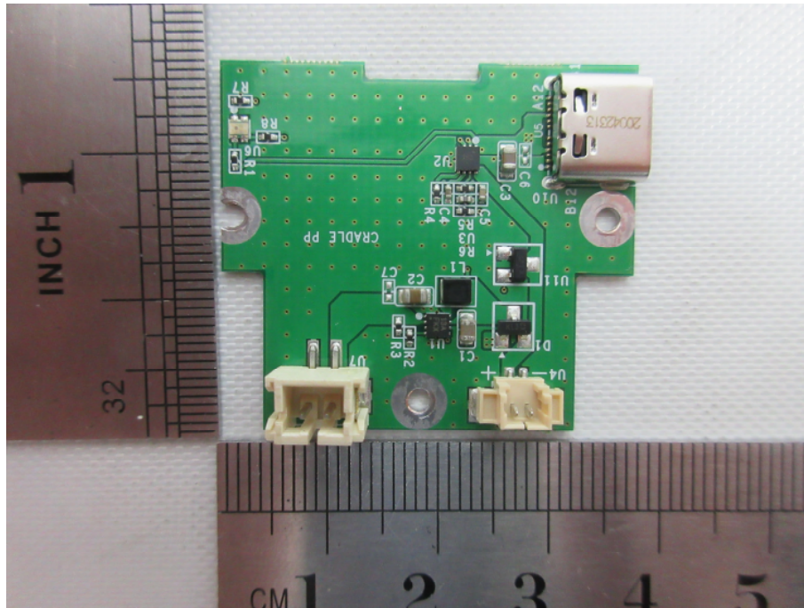
Cradle_Main board_Front
